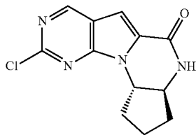
Intermediate 1N
