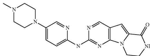
Compound 1
