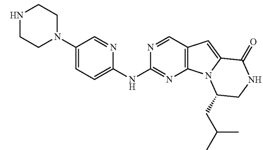
Compound 13
