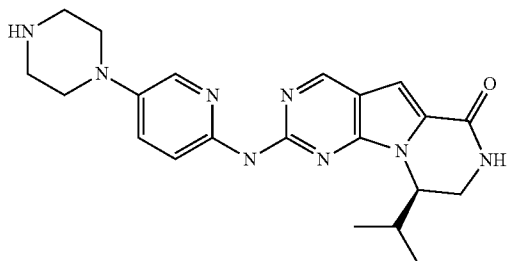
Compound 9
