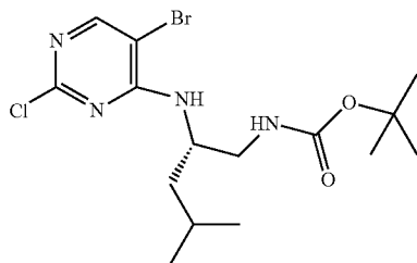
tert-butyl N-[(2S)-2-[(5-bromo-2-chloro-pyrimidin-4-yl)amino]-4-methyl-pentyl]carbamate
