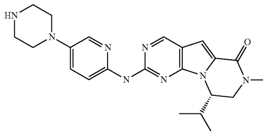
Compound 11
