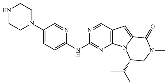
Compound 19
