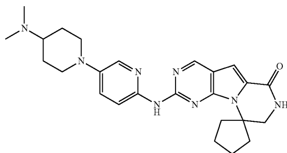
Compound 45
