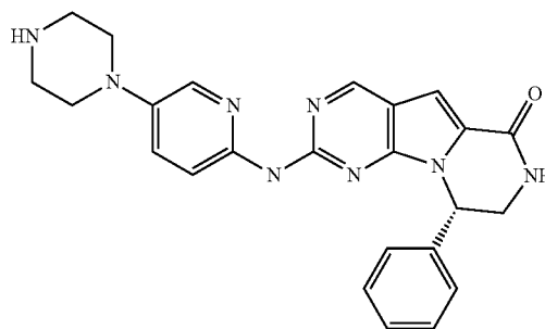
Compound 23
