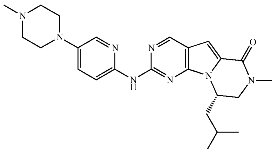
Compound 14
