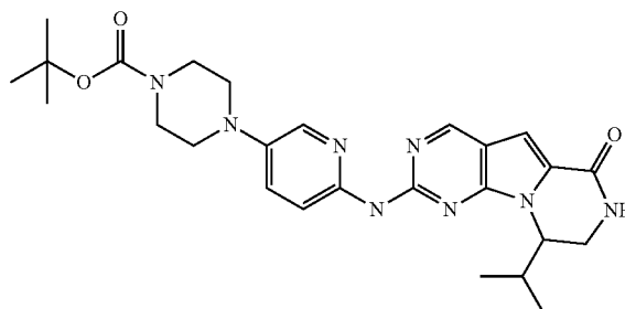
Compound 6
