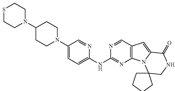
Compound 43
