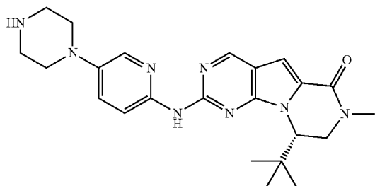
Compound 21
