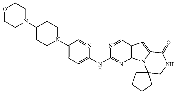
Compound 39
