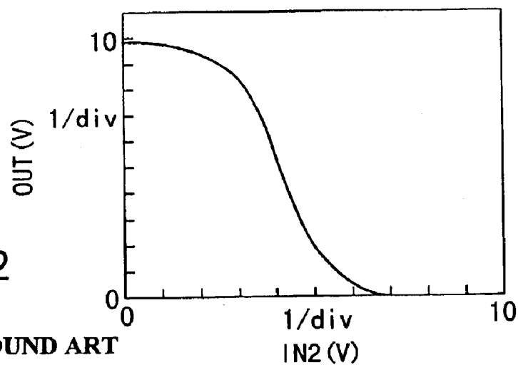
FIG. 11 BACKGROUND ART
