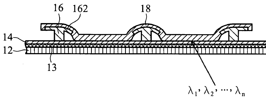
FIG. 1B ( RELATED ART )
