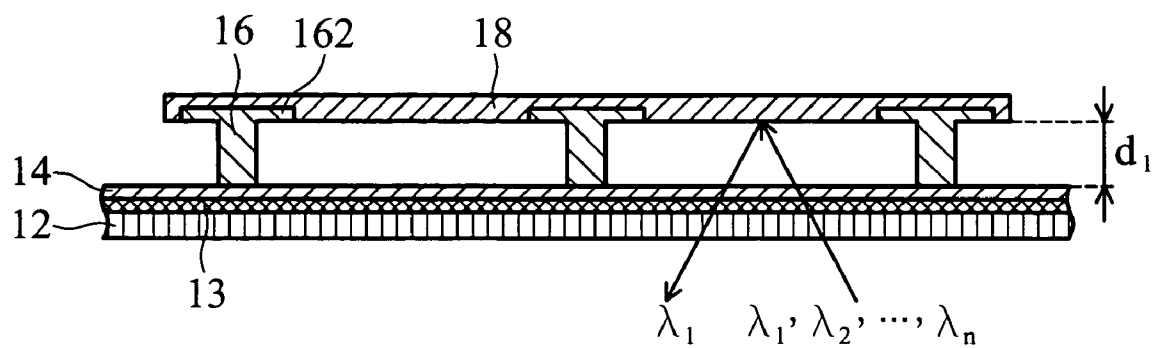
FIG. 1A ( RELATED ART )
