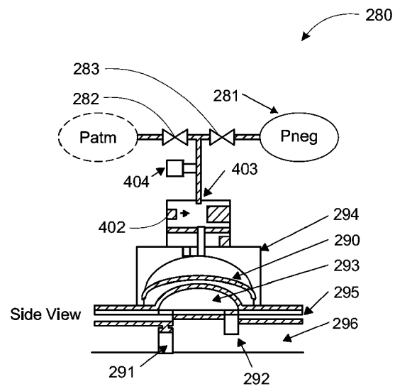
Figure 1: Example Active Fill/Passive Empty Pumping AVS
