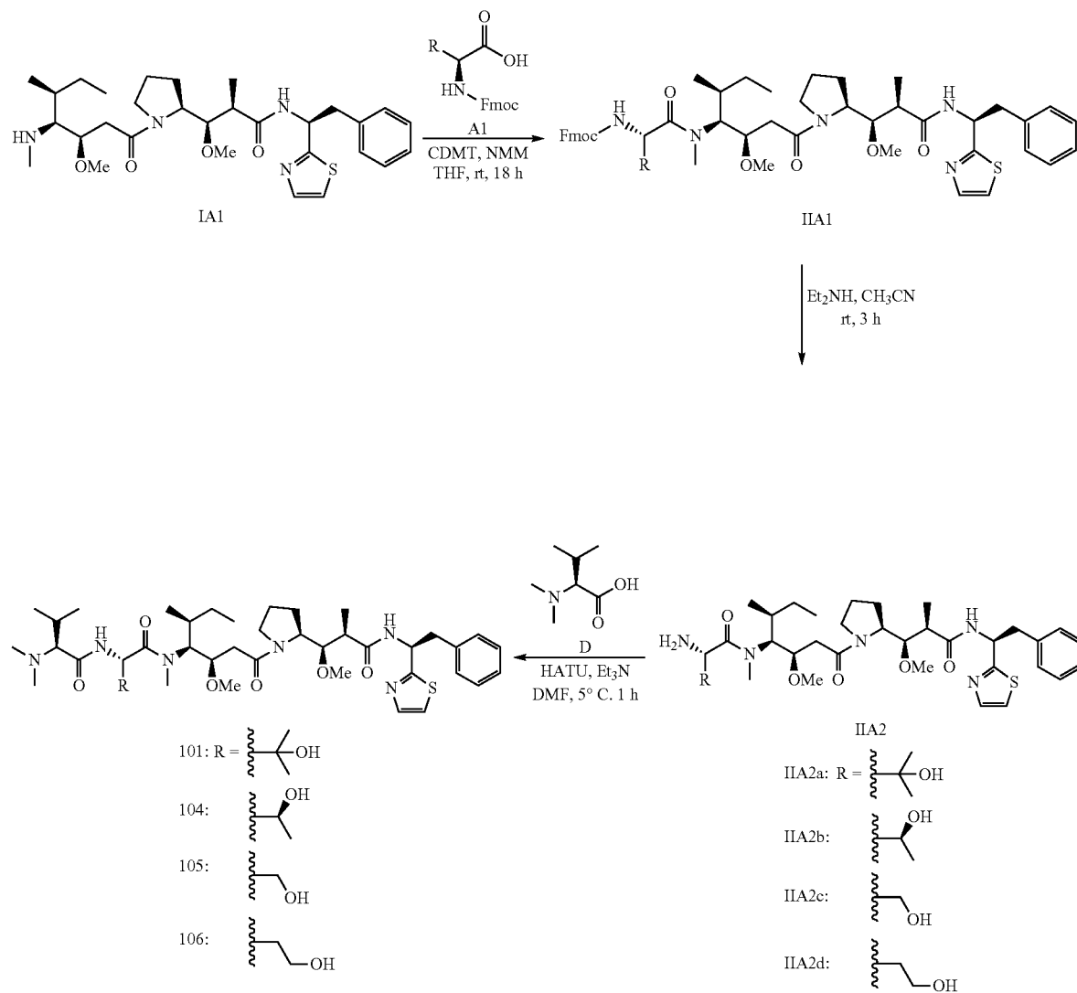
Scheme I-A1:
