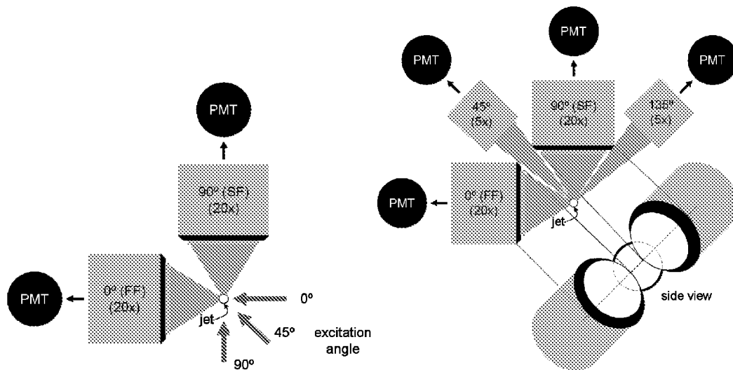
Figure 31. A: Schematic (top view) of standard orthogonal detection layout for sperm DNA content analysis 0° and 90°, but with additional excitation angles of 45° and 90° over the typical 0° only B: quad detector layout (top and side view) showing 0°, 45°, 90° and 135° objectives, filters and PMT detectors encircling the jet in a nested configuration.
