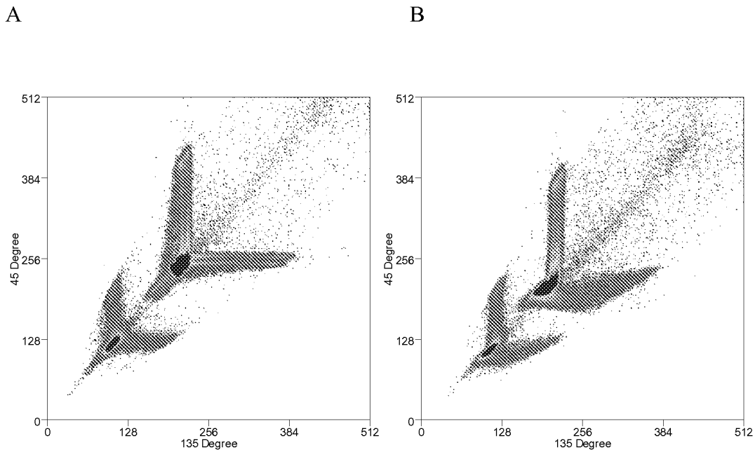
Figure 37. Cell illumination at A) 0°, and B) 45° with respect to 45° and 135 ° detector pair 5 showing orientation dependence on optimal cell excitation and DNA content measurement.
