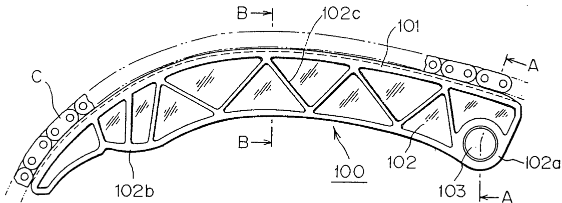
FIG. 10 PRIOR ART
