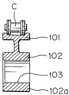
FIG. 11 PRIOR ART
