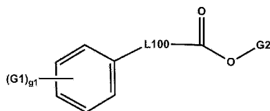
[Chemical Formula B-2]
