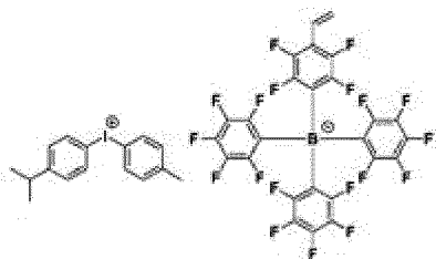
[Chemical Formula 1-1-16]
