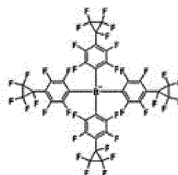
[Chemical Formula 1-2-2]
