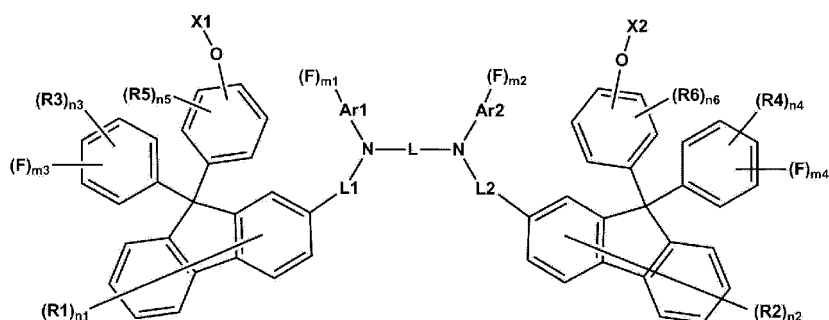
[Chemical Formula 12]
