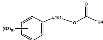
[Chemical Formula B-2]
