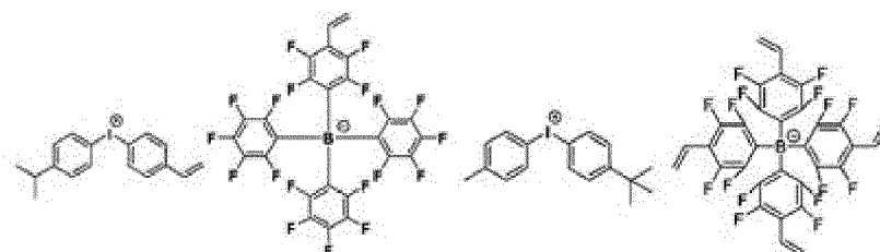
[Chemical Formula 1-1-20]
