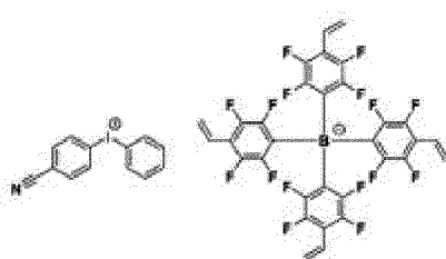
[Chemical Formula 1-1-14]
