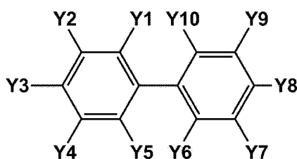
[Chemical Formula B-1]
