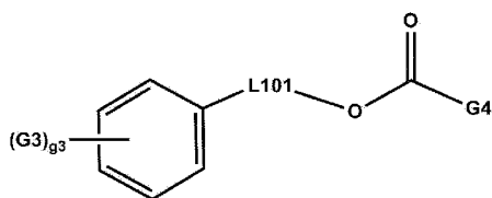
[Chemical Formula B-2]
