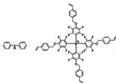
[Chemical Formula 1-1-25]
