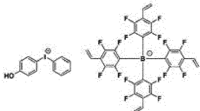
[Chemical Formula 1-1-5]
