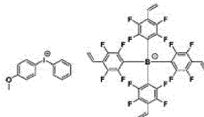
[Chemical Formula 1-1-6]
