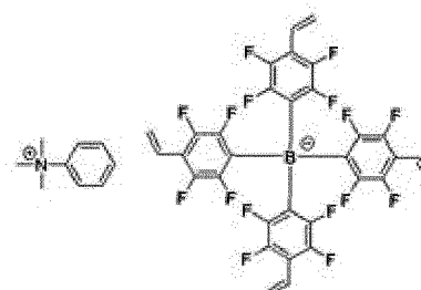
[Chemical Formula 1-3-2]
