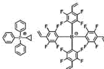
[Chemical Formula 1-5-1]
