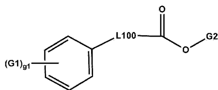
[Chemical Formula B-2]
