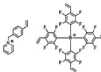
[Chemical Formula 1-3-4]
