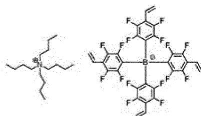
[Chemical Formula 1-3-3]
