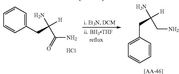
Synthesis of (S)-3-phenyl-propane-1,2-diamine [AA-46]
