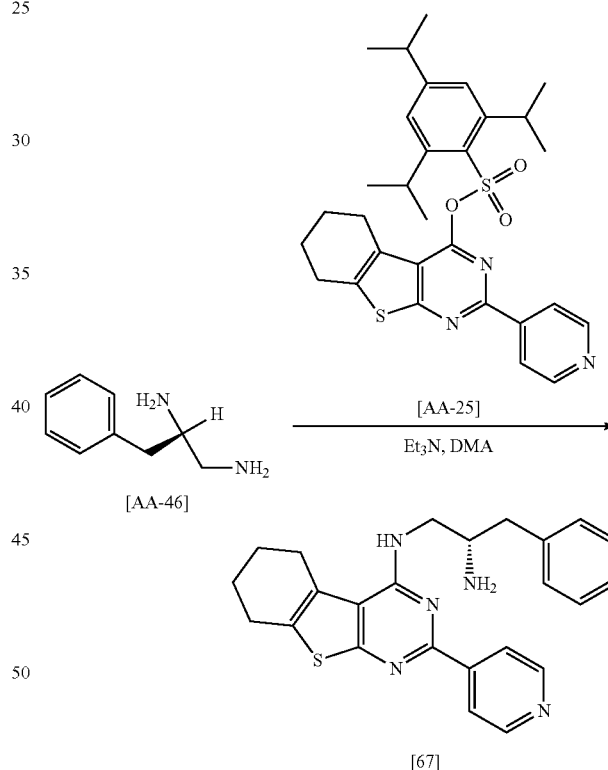
Synthesis of (S)-N*1*-(2-pyridin-4-yl-5,6,7,8-tetrahydro-benzo[4,5]thieno[2,3-d]pyrimidin-4-yl)-butane-1,2-diamine [67]
