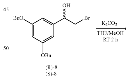
Scheme I
