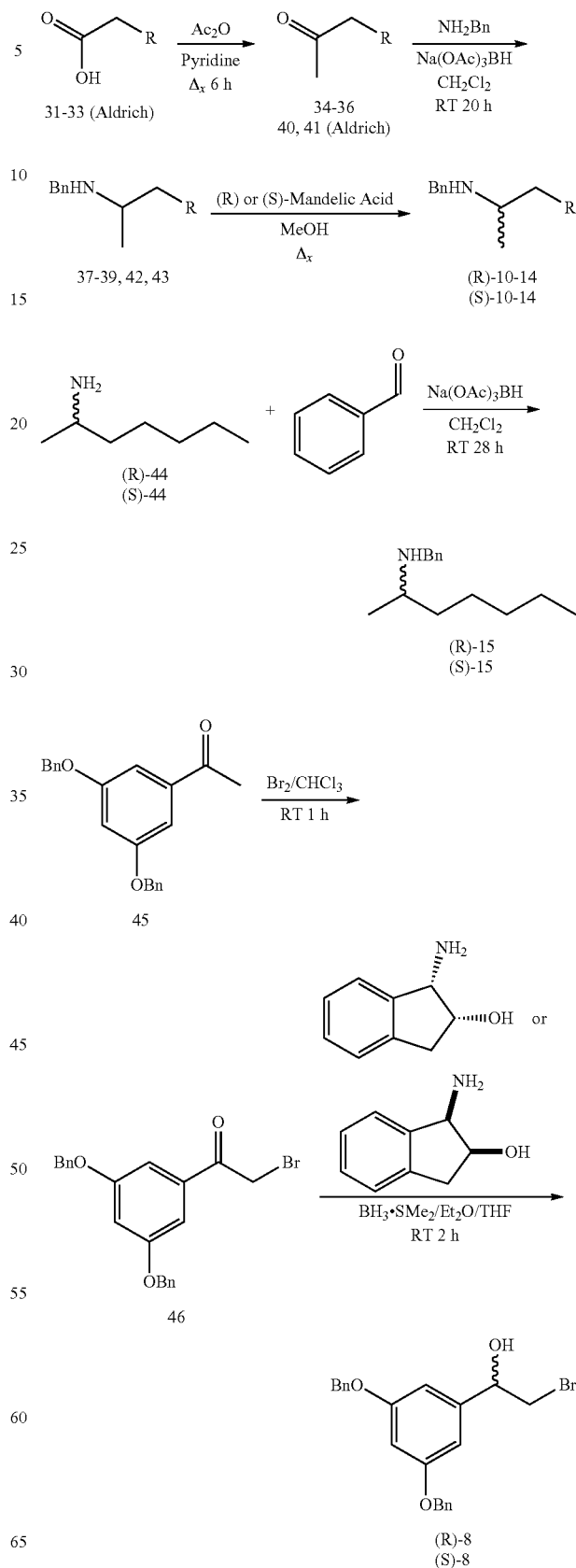
Scheme III
