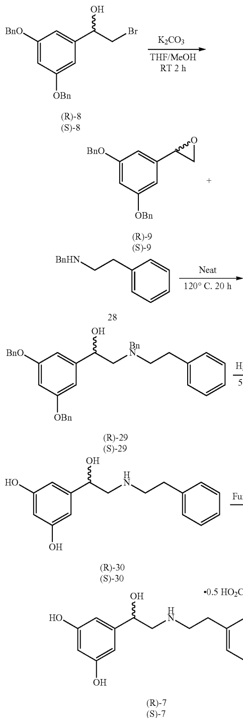
Scheme II
