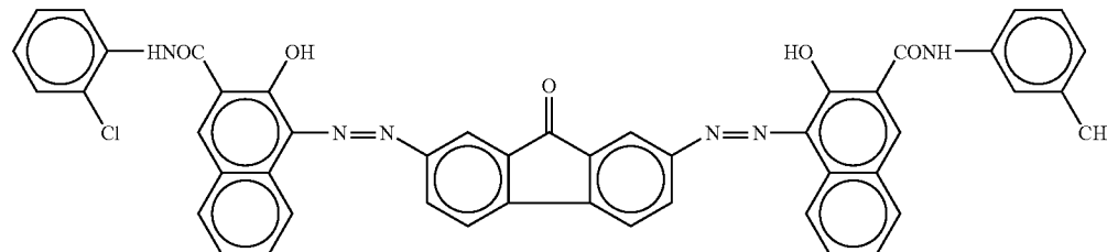
Chemical Structure 4
