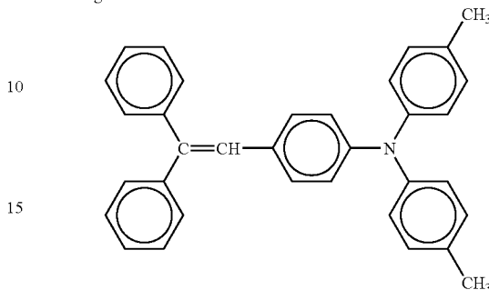
Chemical structure 5
