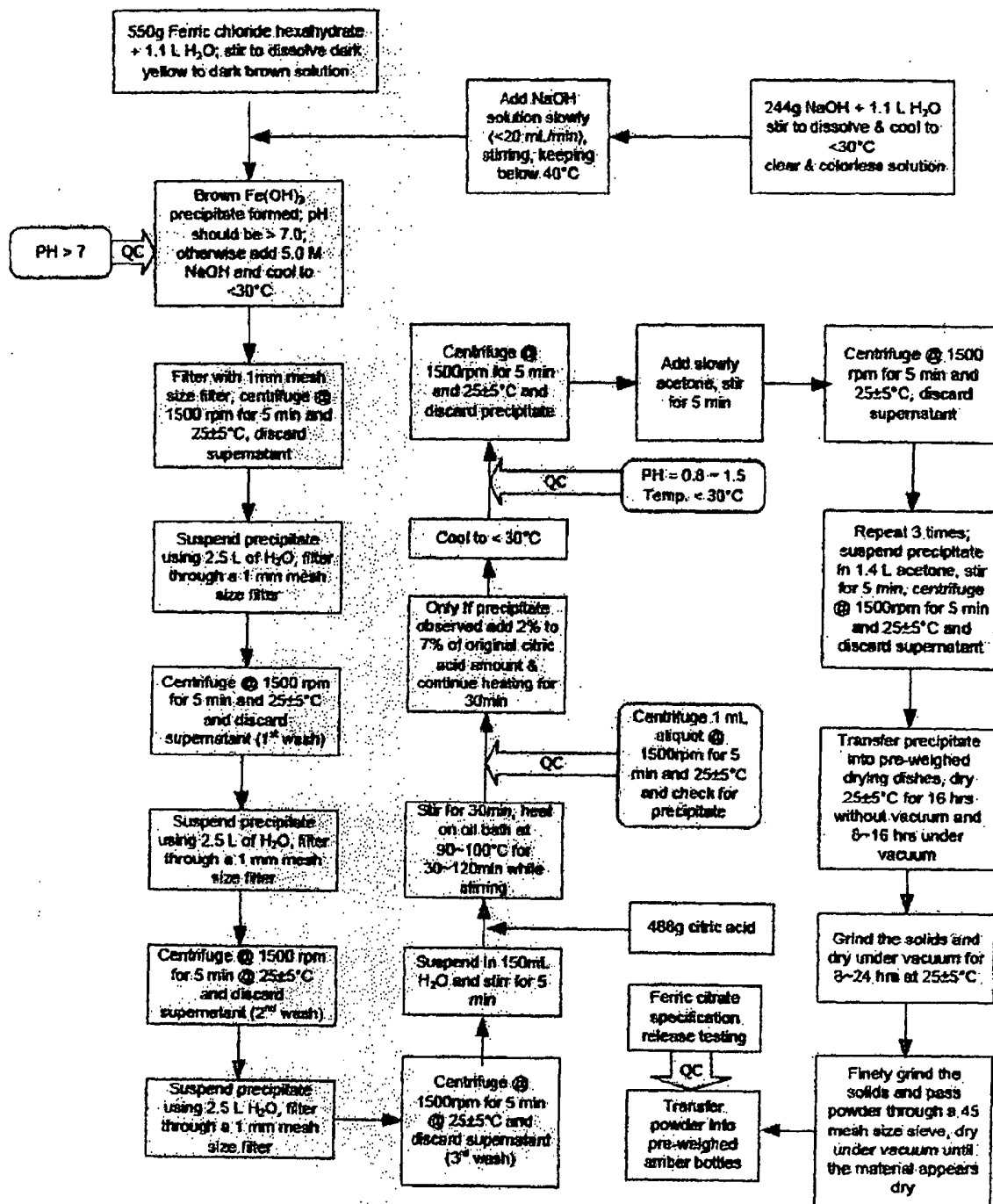
Figure 2 Pharmaceutical-Grade Ferric Citrate manufacture Flow Chart
