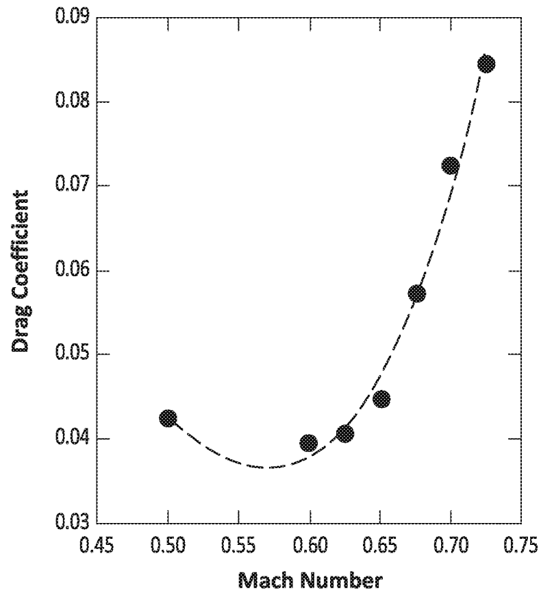
Drag Coefficient vs. Mach Number
