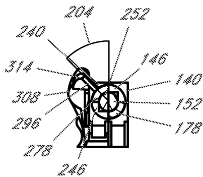
SECTION P-P Scale 2:1
