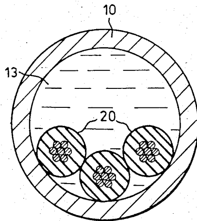
PRIOR ART FIG. 2b
