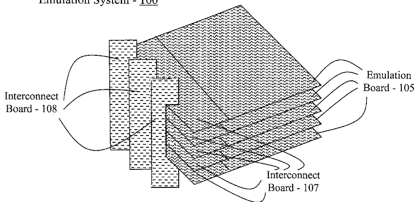
Emulation System - 100
