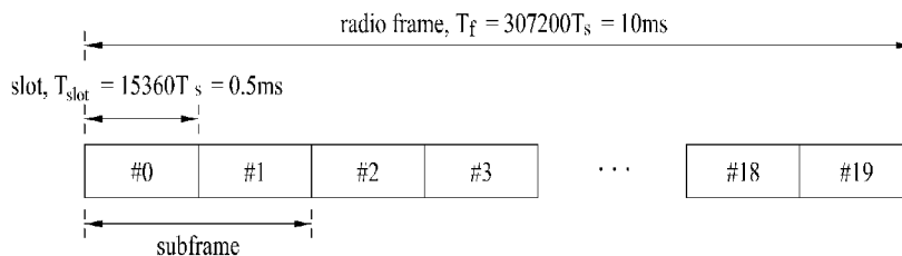
(a) Frame structure type-1
