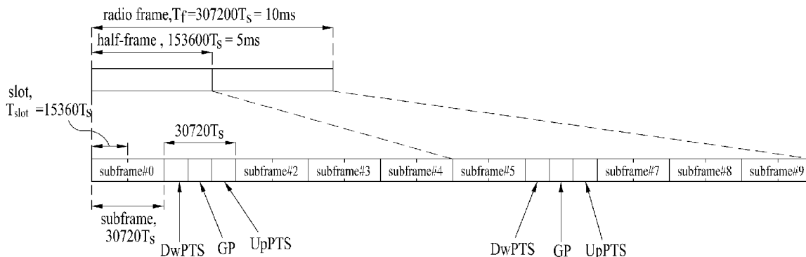
(b) Frame structure type-2
