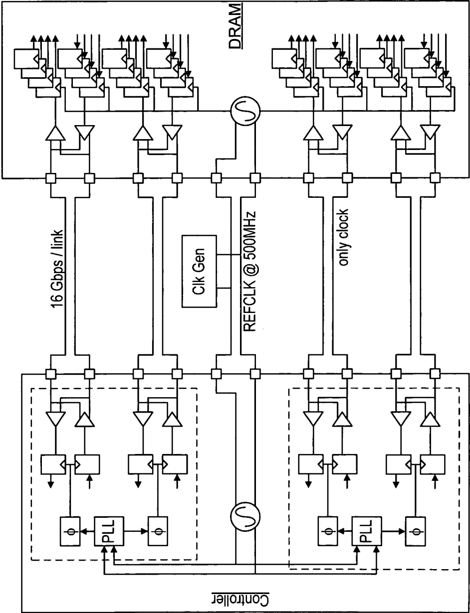
TBI System Clocking and Signaling
