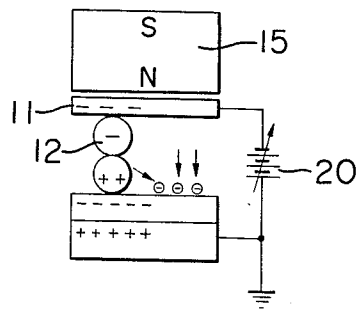
FIG. 12 PRIOR ART
