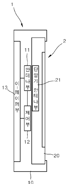
11 ... Antenna unit 12 ... Control unit 13 ... E-paper unit 21 ... Terminal antenna unit
