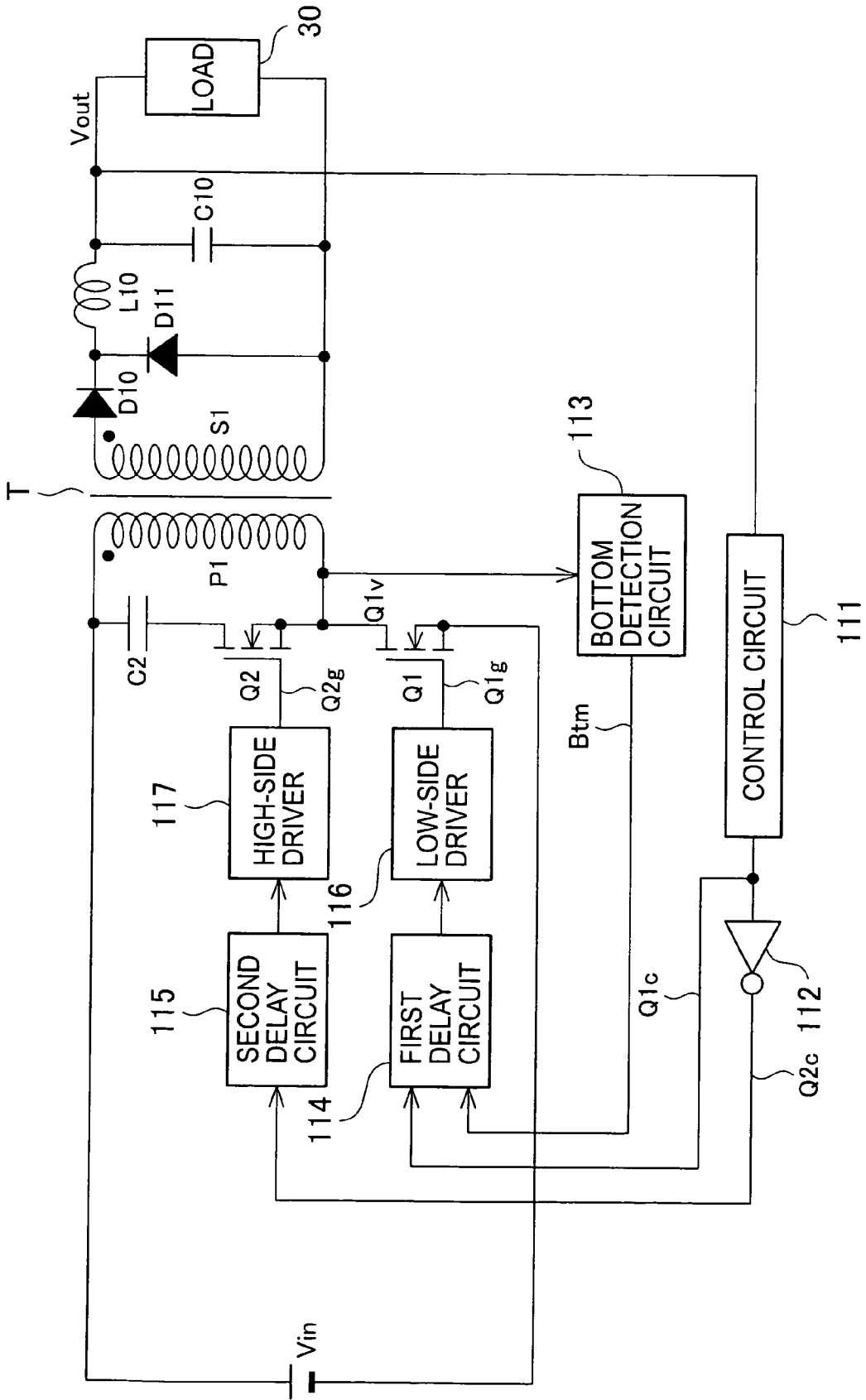
FIG. 1 PRIOR ART
