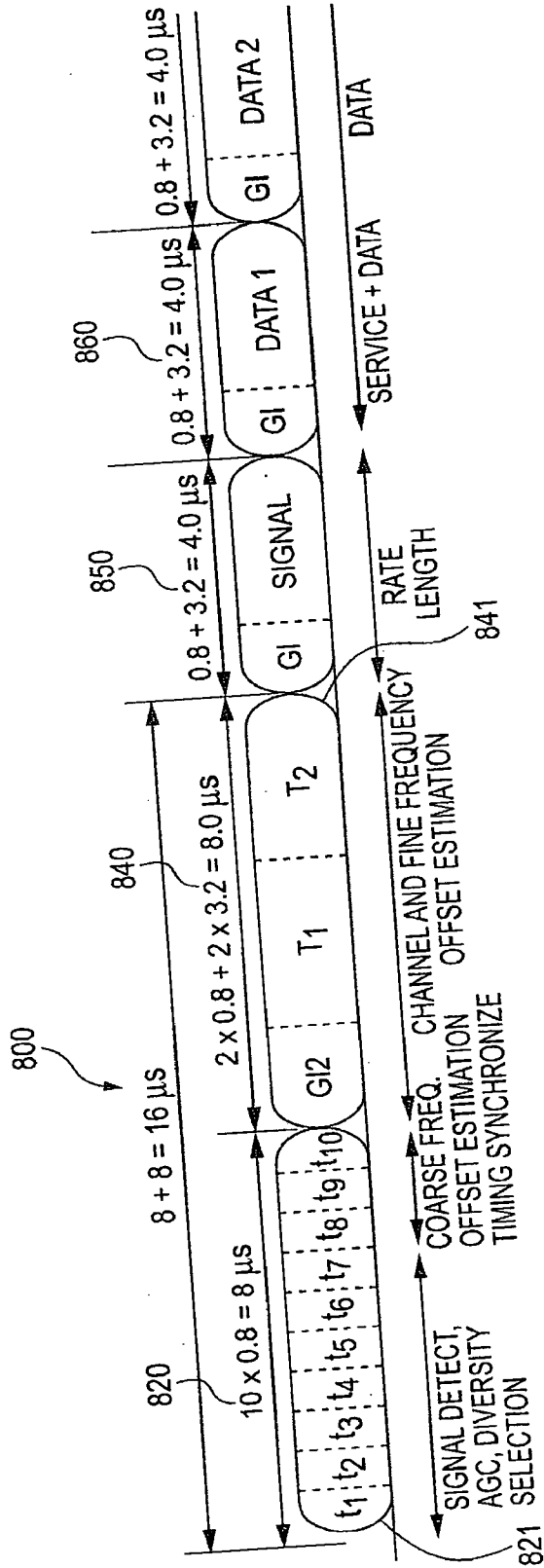
FIG. 8 PRIOR ART
