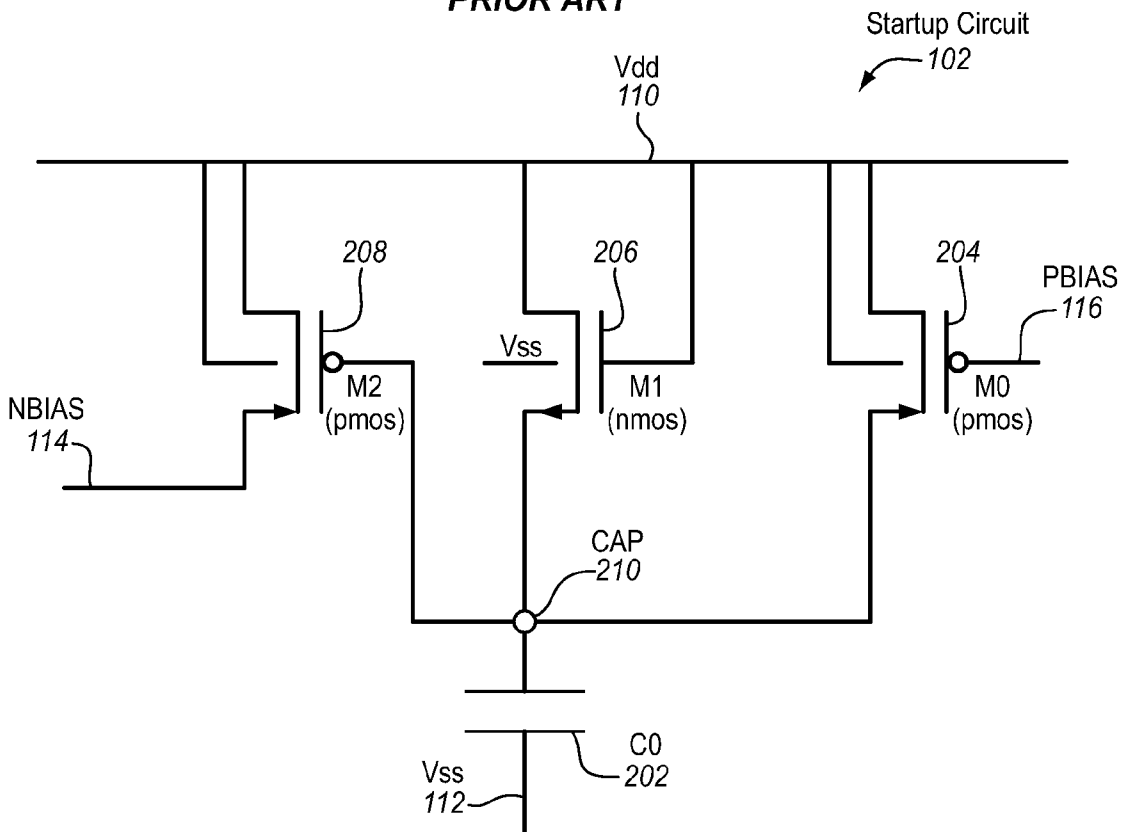
FIG. 2 PRIOR ART
