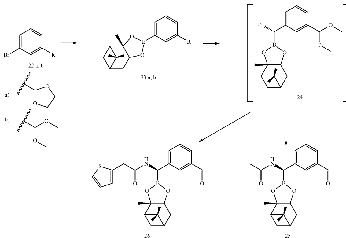
Scheme 3. Steps in the synthesis of compound 26.
