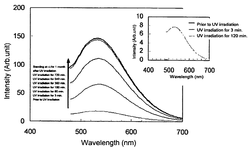
(b) Fluorescence emission spectra
