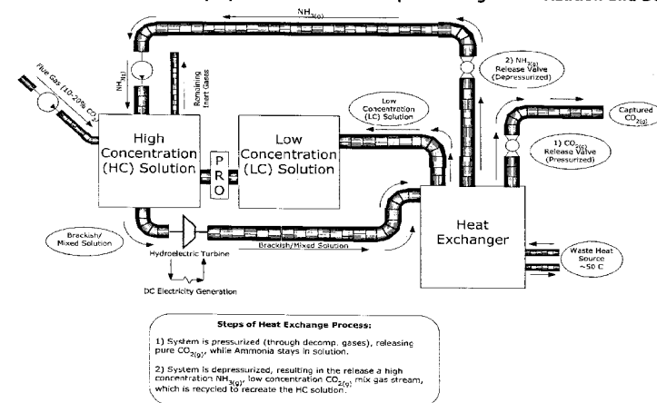
PRO Waste Heat Recovery System with Carbon Capture using Pressurization and Depressurization
