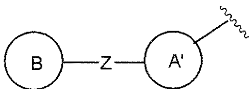
[Chemical Formula 4]
