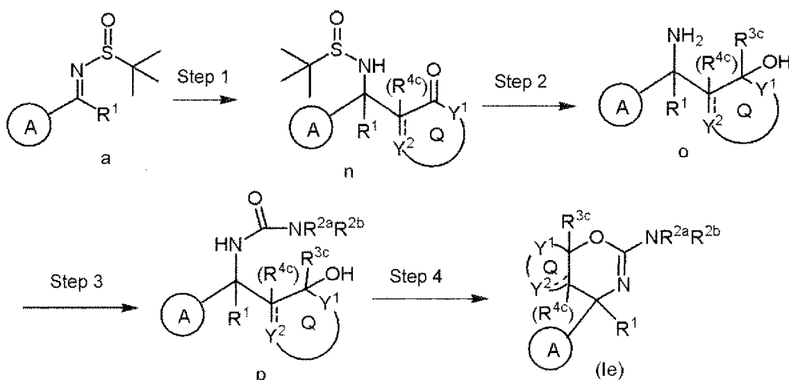
[Chemical Formula 43]
