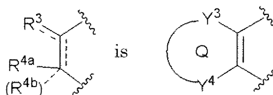
[Chemical Formula 21]
