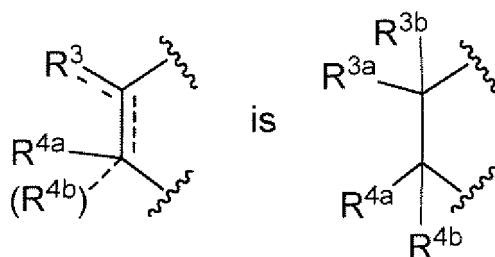
[Chemical Formula 3]
