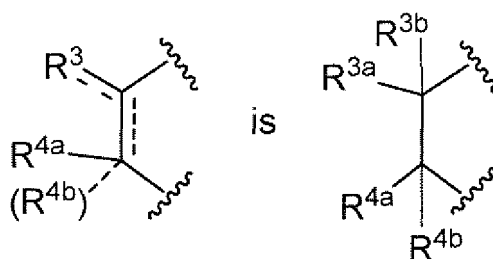
[Chemical Formula 7]
