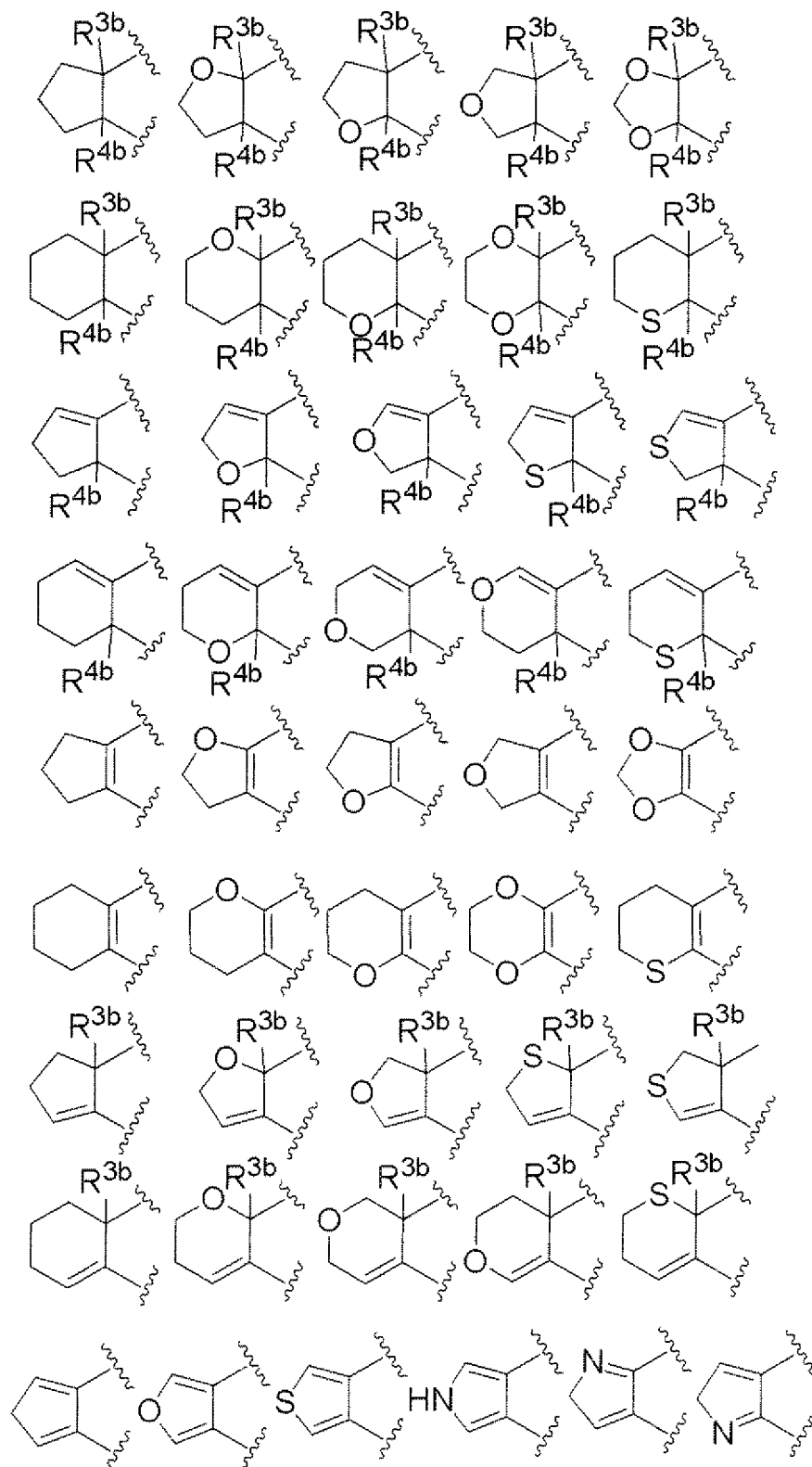
[Chemical Formula 28]
