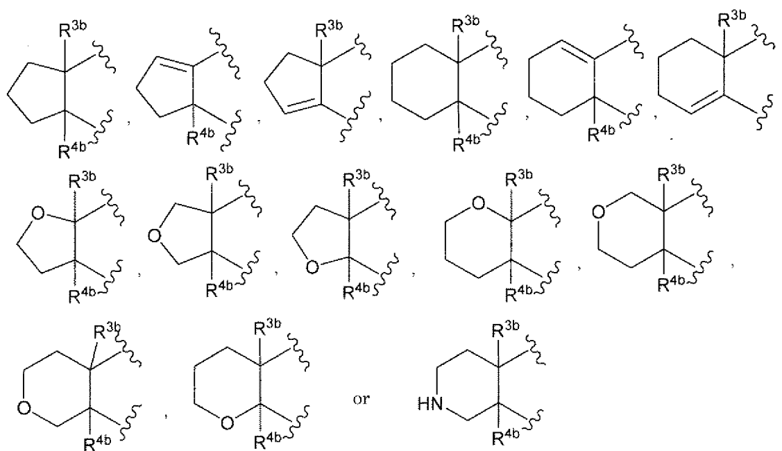
[Chemical Formula 67]
