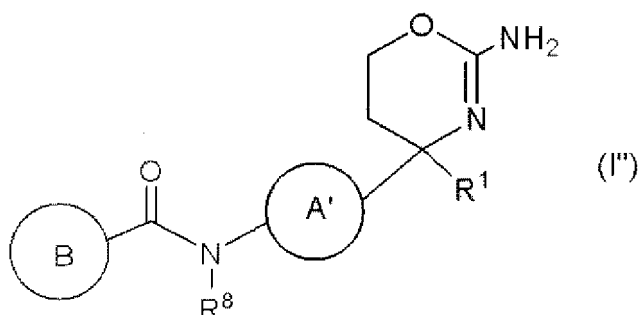
[Chemical Formula 72]
