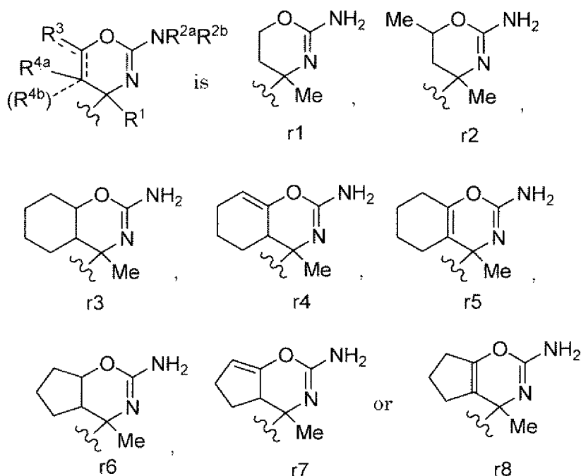
[Chemical Formula 74]
