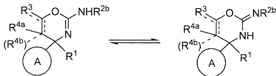
[Chemical Formula 35]
