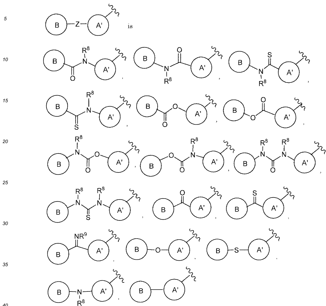
[Chemical Formula 52]
