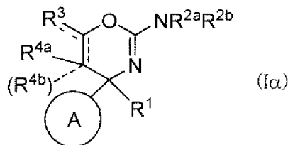
[Chemical Formula 9]
