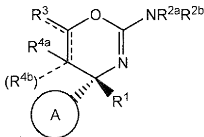
[Chemical Formula 37]
