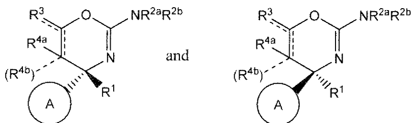
[Chemical Formula 36]
