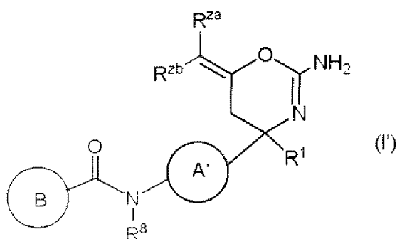
[Chemical Formula 71]
