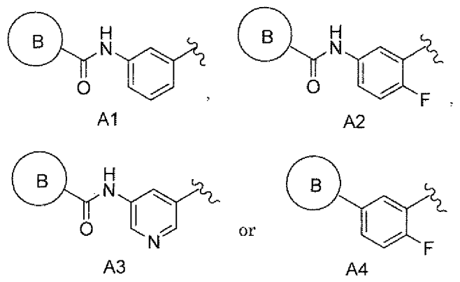
[Chemical Formula 75]
