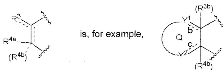
[Chemical Formula 66]
