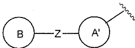
[Chemical Formula 46]
