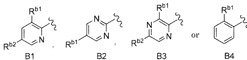
[Chemical Formula 76]
