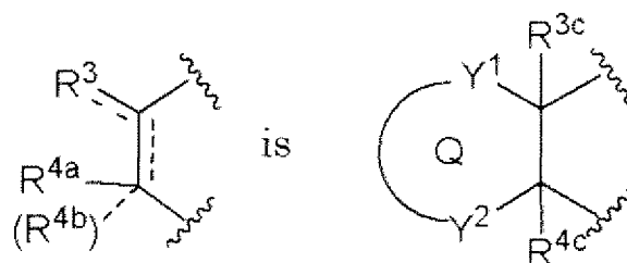
[Chemical Formula 20]
