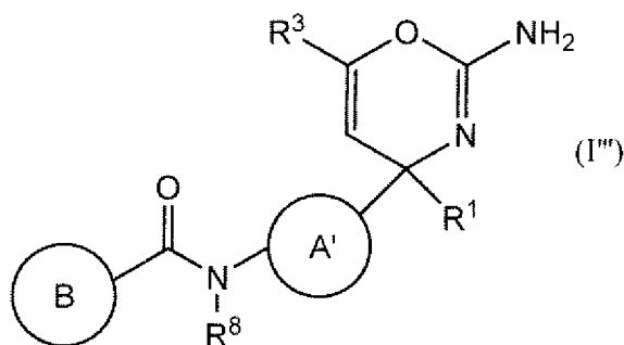
[Chemical Formula 73]
