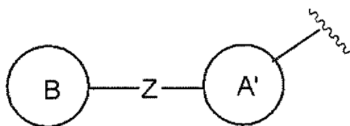
[Chemical Formula 8]
