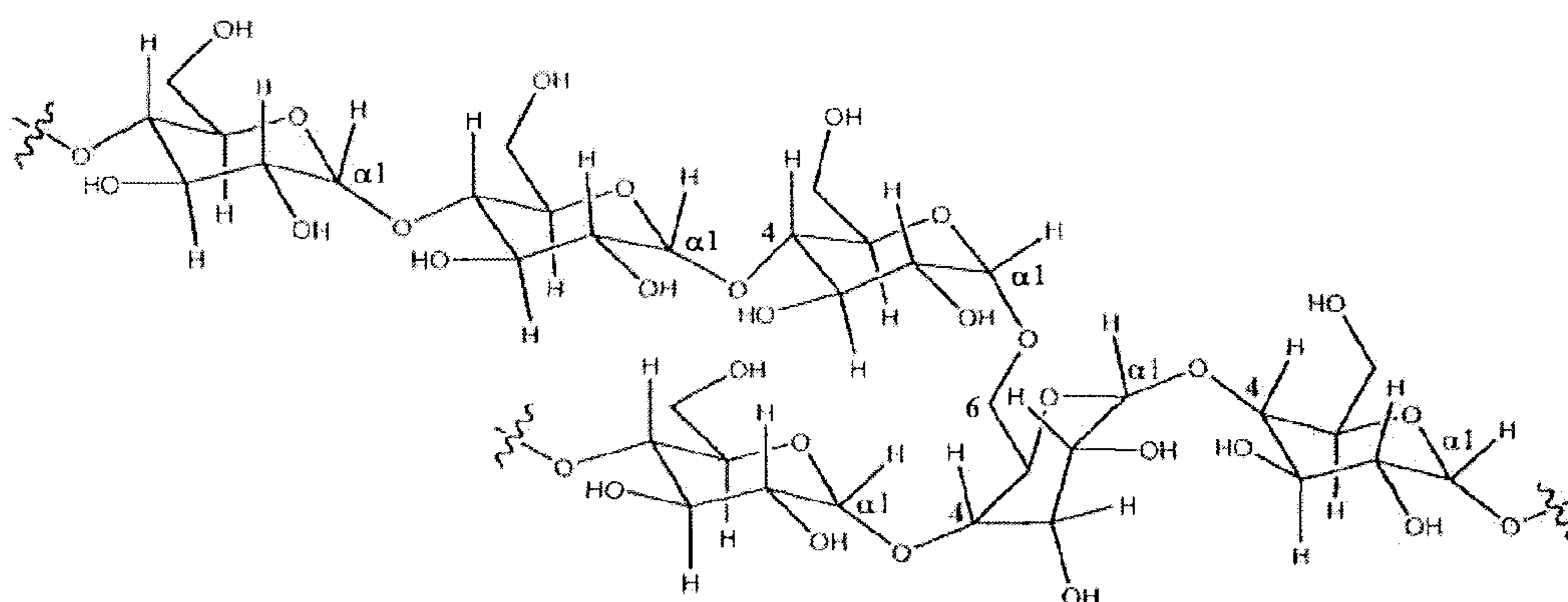
Figure 3. Representative partial structure of amylopectin
