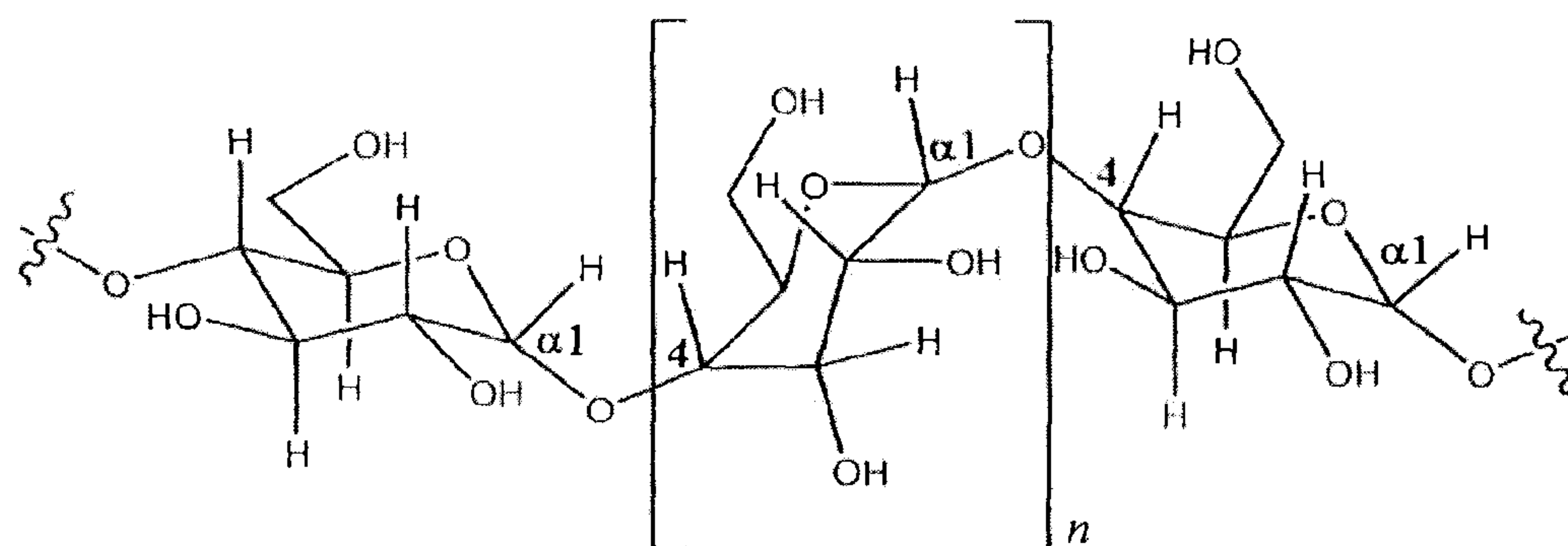
Figure 2. Representative Partial Structure of Amylose
