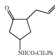
Step 1: benzyl 3-allyl-4-oxocyclopentylcarbamate
