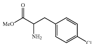
Step 1: Methyl 2-amino-3-(4-chlorophenyl)propanoate hydrochloride
