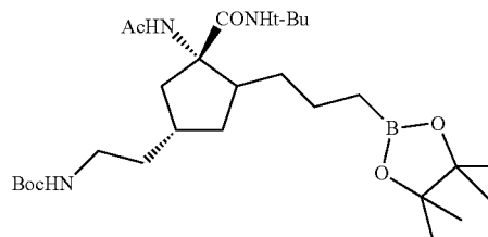
Step 5: tert-butyl 2-((1R,3S)-3-acetamido-3-(tert-butylcarbamoyl)-4-(3-(4,4,5,5-tetramethyl-1,3,2-dioxaborolan-2-yl)propyl)cyclopentyl)ethylcarbamate
