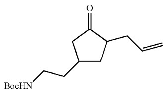
Step 3: tert-butyl 2-(3-allyl-4-oxocyclopentyl)ethylcarbamate
