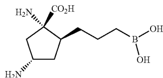
Step 7: (1S,2S,4S)-1,4-diamino-2-(3-boronopropyl)cyclopentanecarboxylic acid (Racemic)
