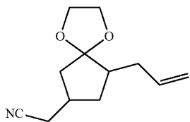
Step 2: 2-(9-allyl-1,4-dioxaspiro[4.4]nonan-7-yl)acetonitrile
