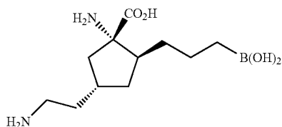
Step 6: (1S,2S,4R)-1-amino-4-(2-aminoethyl)-2-(3-boronopropyl) cyclopentanecarboxylic acid
