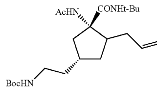
Step 4: tert-butyl 2-((1R,3S)-3-acetamido-4-allyl-3-(tert-butylcarbamoyl)cyclopentyl)ethylcarbamate
