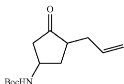
Step 4: tert-butyl 3-allyl-4-oxocyclopentylcarbamate
