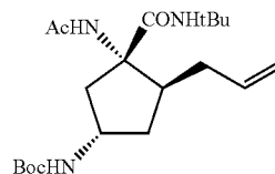
Step 5: tert-butyl (1S,3S,4S)-3-acetamido-4-allyl-3-(tert-butylcarbamoyl) cyclopentylcarbamate
