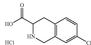
Step 4: 7-chloro-1,2,3,4-tetrahydroisoquinoline-3-carboxylic acid hydrochloride
