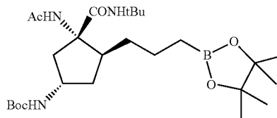
Step 6: tert-butyl (1S,3S,4S)-3-acetamido-3-(tert-butylcarbamoyl)-4-(3-(4,4,5,5-tetramethyl-1,3,2-dioxaborolan-2-yl)propyl)cyclopentylcarbamate
