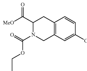
Step 3: 2-Ethyl 3-methyl 7-chloro-3,4-dihydroisoquinoline-2,3(1H)-dicarboxylate
