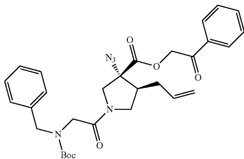
Step 2: 2-Oxo-2-phenylethyl (3R,4S)-4-allyl-3-azido-1-[N-benzyl-N-(tert-butoxycarbonyl)glycyl]pyrrolidine-3-carboxylate
