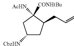
Step 2: benzyl (1S,3S,4S)-3-acetamido-4-allyl-3-(tert-butylcarbamoyl)cyclopentylcarbamate
