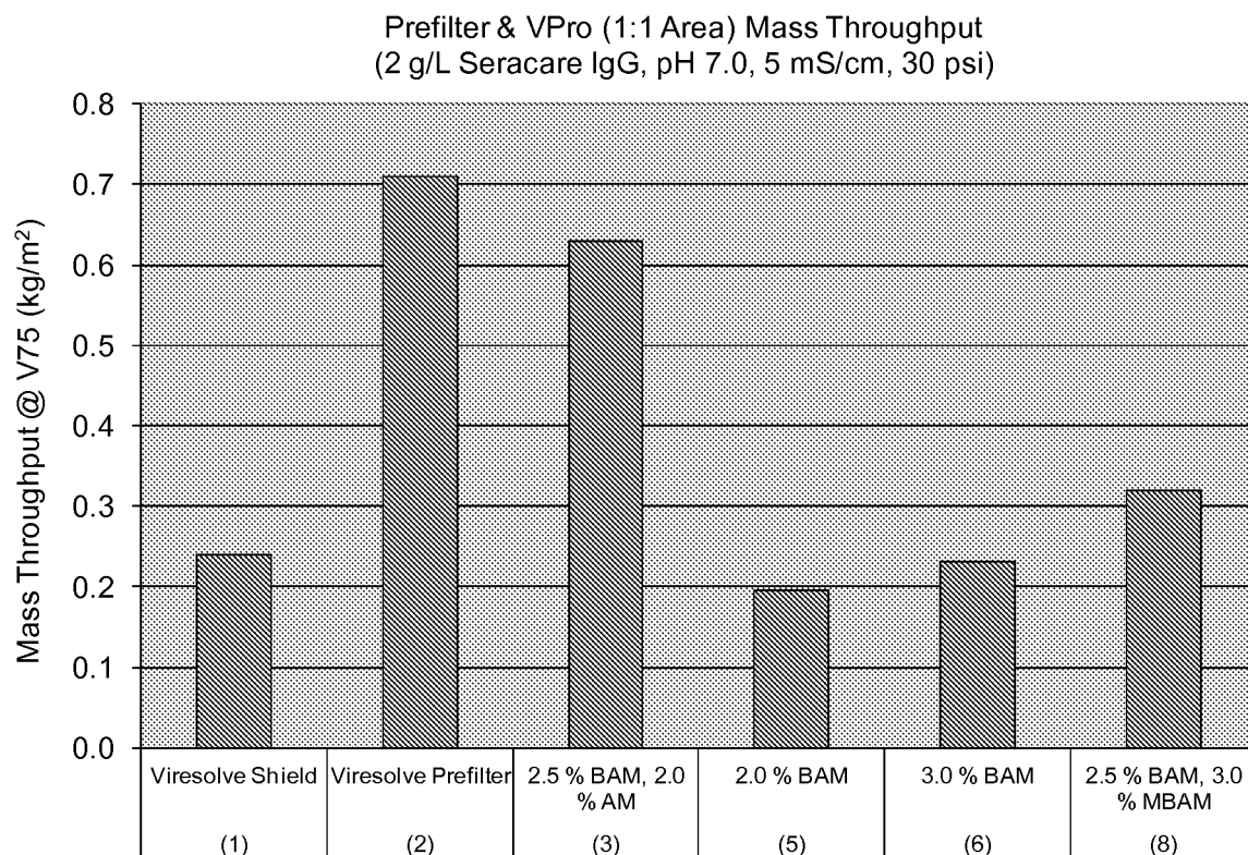
Figure 10. Performance of Acrylamide-containing hydrophobic prefilters in comparison to currently available commercial prefilters and prefilters without Acrylamide at pH 7.0, 5 mS/cm.
