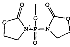
Mixed phosphorus acid anhydride
