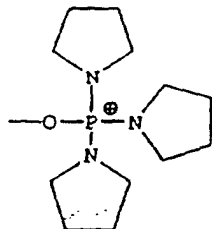
Acyl phosphonium mixed anhydride
