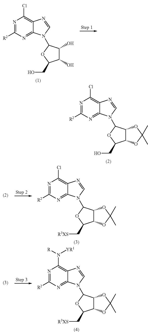
REACTION SCHEME 1
