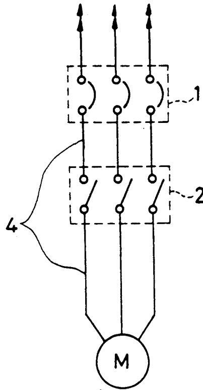
FIG. 24 (Prior Art)
