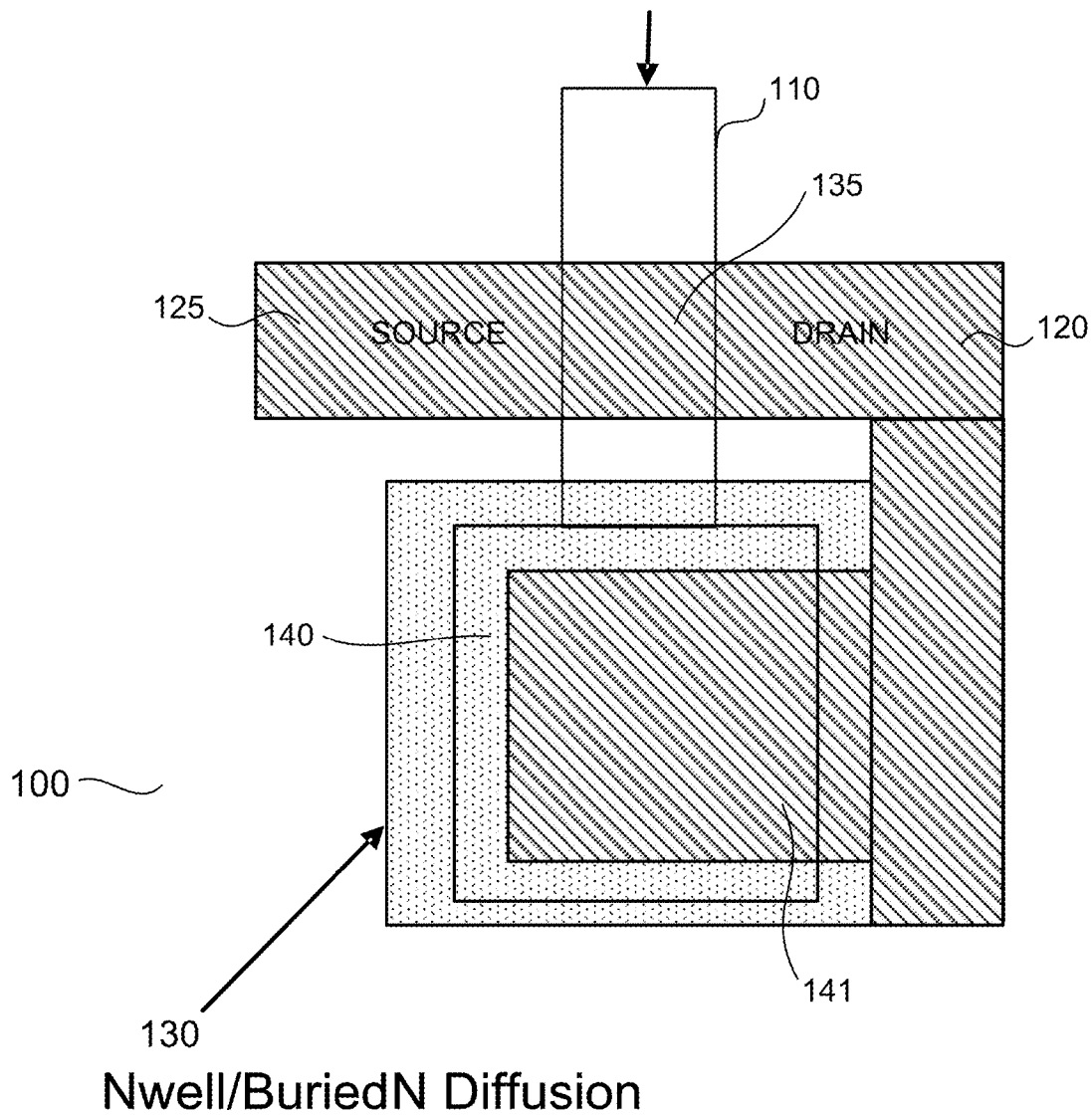
FIG. 1 Floating Gate
