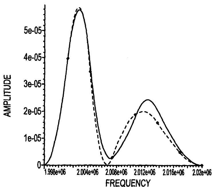
FIG.48 ——— ACTUAL F(f) - - - - - F(f) : DISTRIBUTION CALC'D USING |a| AND |x| CALC'D f ..... SEGMENT ENDPOINTS FOR PREDICTED QUADRATIC
