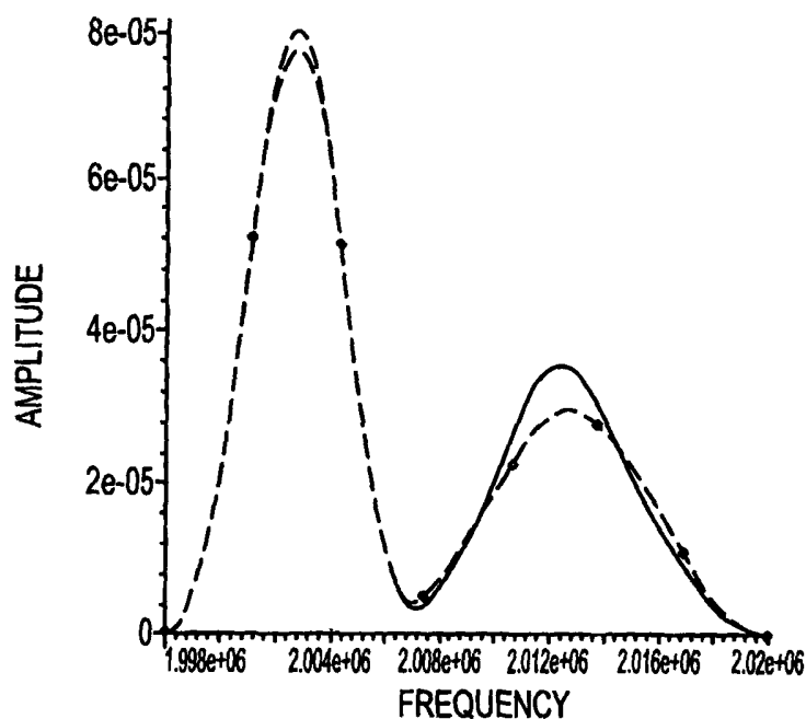
FIG.47 ——— ACTUAL G(f) - - - - - G(f) : DISTRIBUTION CALC'D USING |a| AND |x| CALC'D f ..... SEGMENT ENDPOINTS FOR PREDICTED QUADRATIC
