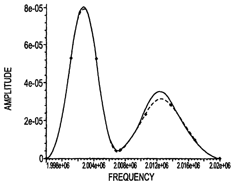
FIG.50 ——— ACTUAL G(f) - - - - - G(f) : DISTRIBUTION CALC'D USING |a| AND |x| CALC'D F . . . . . SEGMENT ENDPOINTS FOR PREDICTED QUADRATIC
