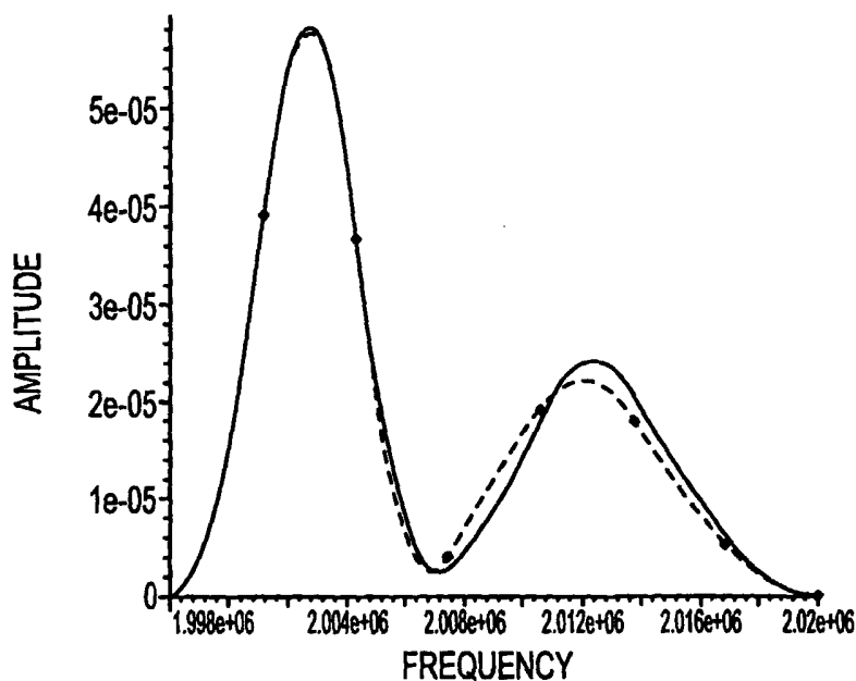
FIG.51 ——— ACTUAL F(f) - - - - - F(f) : DISTRIBUTION CALC'D USING |a| AND |x| CALC'D F . . . . . SEGMENT ENDPOINTS FOR PREDICTED QUADRATIC
