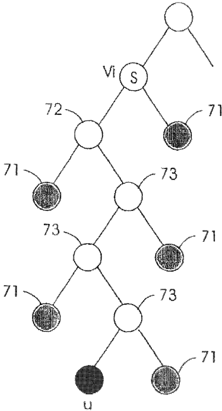
FIG. 14 - ASSIGNMENT OF LABELS SUBSET DIFFERENCE METHOD
