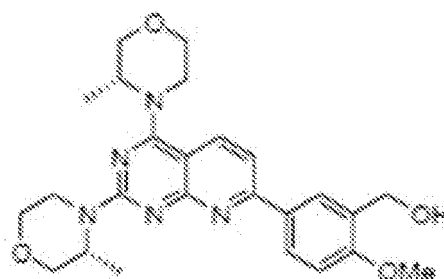
AZD8055
