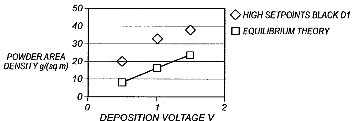
POWDER AREA DENSITY VS. DEPOSITION VOLTAGE
