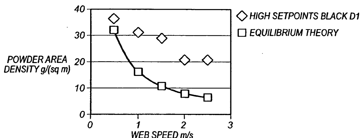
POWDER AREA DENSITY VS. WEB SPEED
