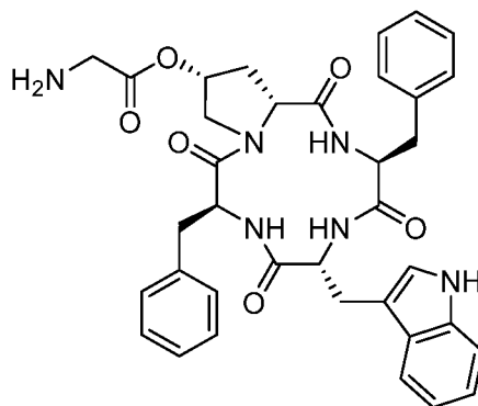
cyclo [Phe- cis -D-Hyp(Gly) 2 -Phe-D-Trp] (JVA 4102);
