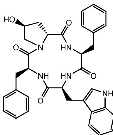
cyclo [Phe- trans -D-Hyp-Phe-Trp],
