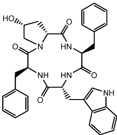
cyclo [Phe- cis -D-Hyp-Phe-D-Trp],
