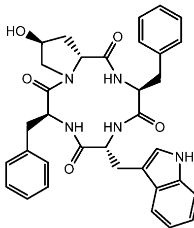
cyclo [Phe- trans -D-Hyp-Phe-D-Trp],
