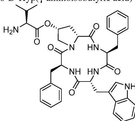
cyclo [Phe- cis -D-Hyp(γ-aminoisobutyric acid) 2 -Phe-D-Trp];
