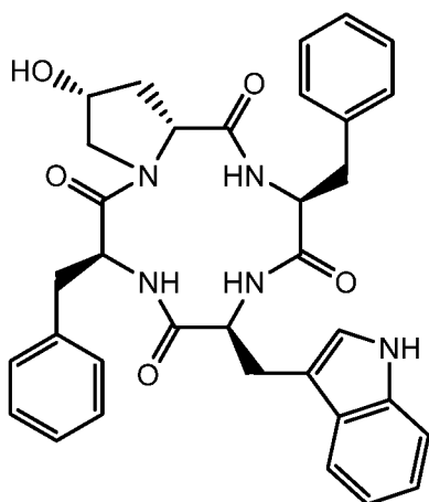
cyclo [Phe- cis -D-Hyp-Phe-Trp],
