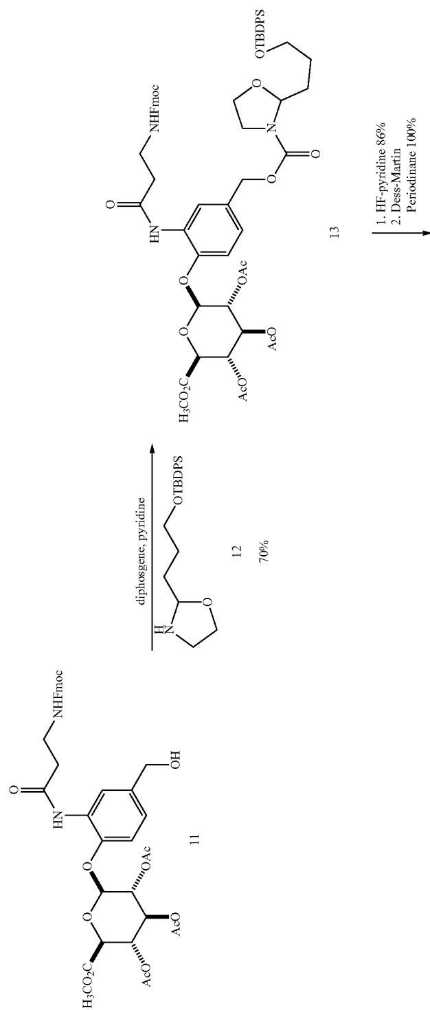
Scheme 4
