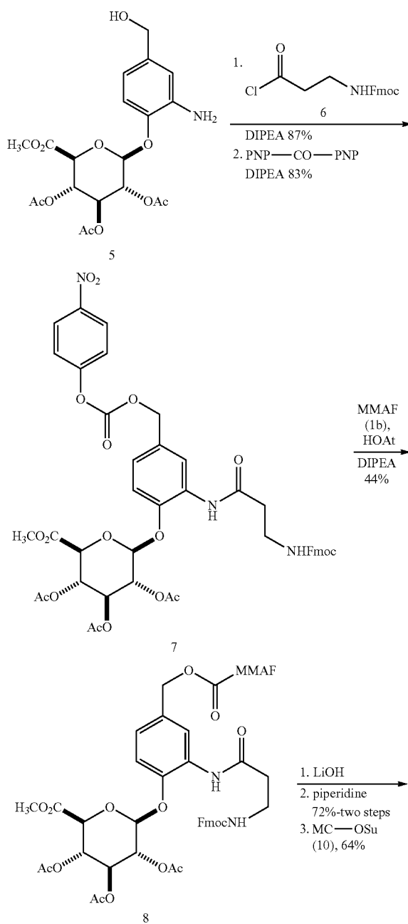
Scheme 3
