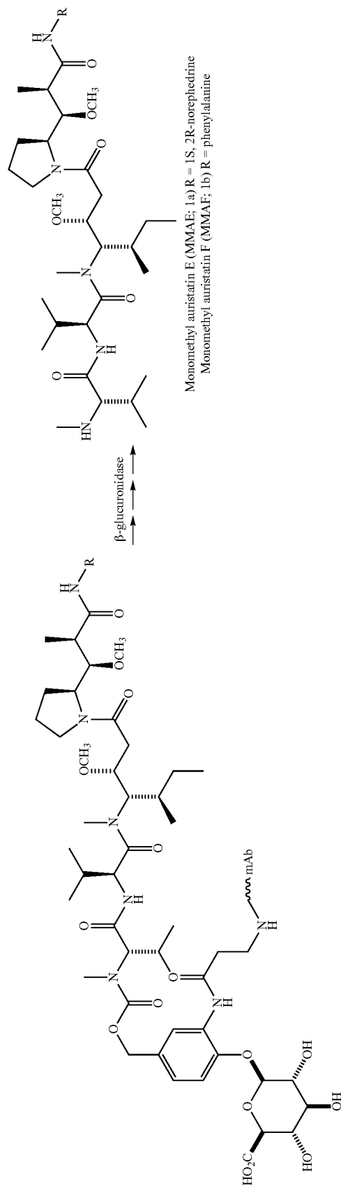
Scheme 2.
