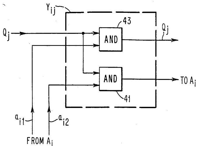
FIG. 5.1 STATION SWITCH
