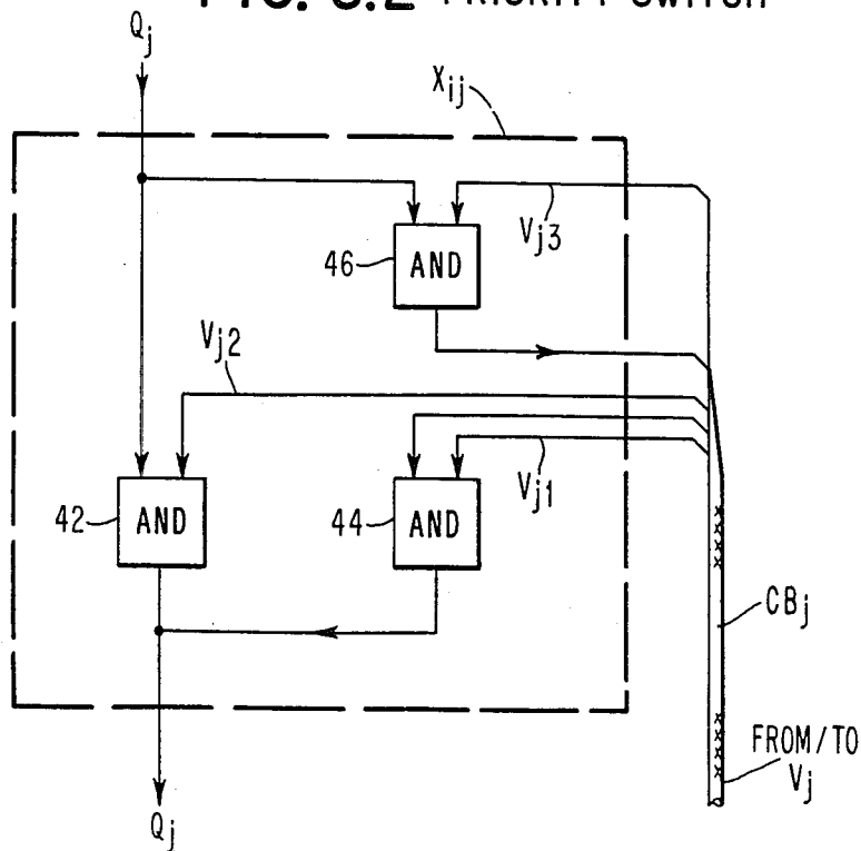
FIG. 5.2 PRIORITY SWITCH
