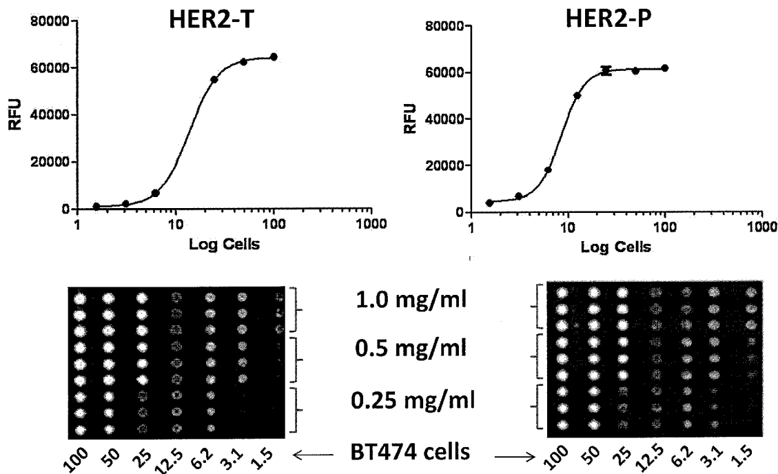
Standard Curve for HER2 quantitation
