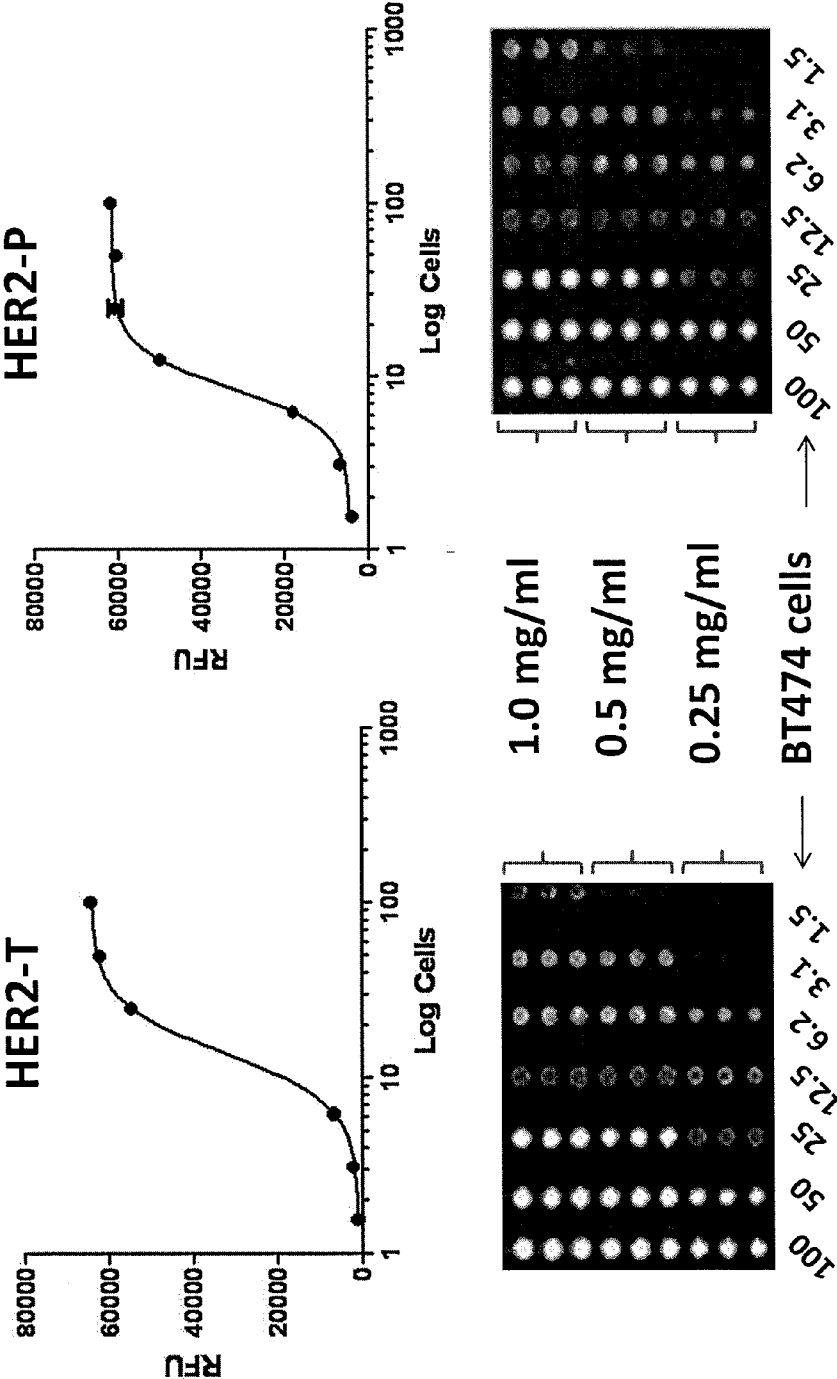
Standard Curve for HER2 quantitation
