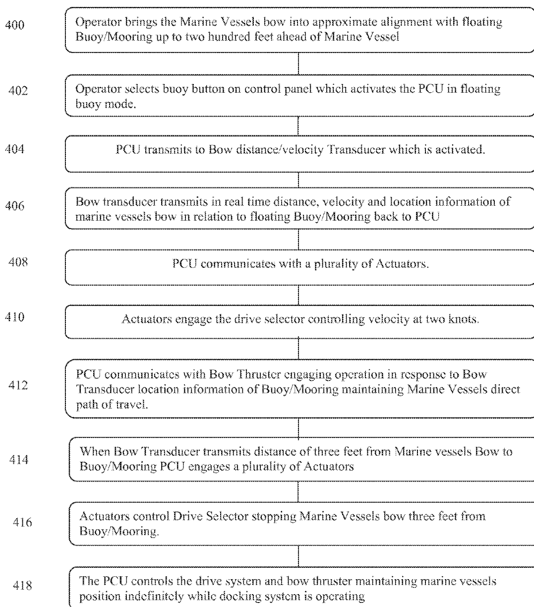
FLOATING BUOY/MOORING OPERATION Fig.8
