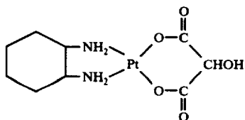
hydroxymalonato (1,2-diaminocyclohexane) platinum (II)
