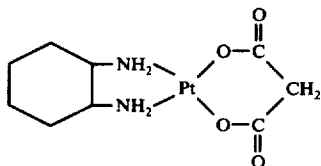
malonato (1,2-diaminocyclohexane) platinum (II)
