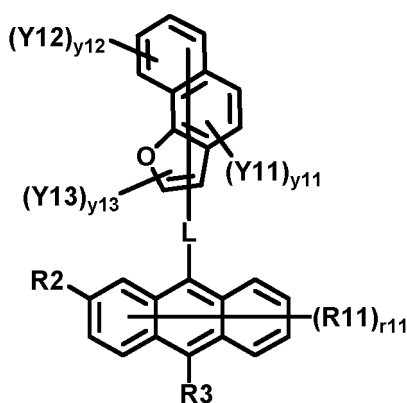
[Chemical Formula 1-5]
