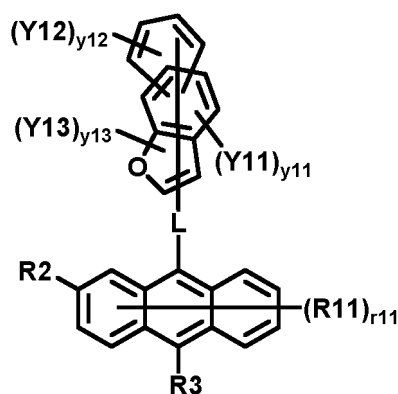
[Chemical Formula 1-2]
