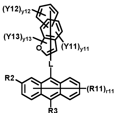
[Chemical Formula 1-2]
