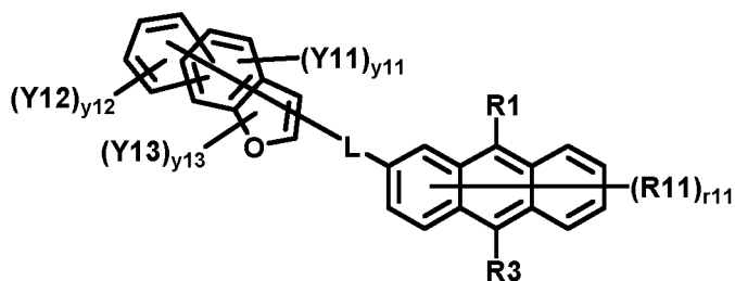
[Chemical Formula 1-3]
