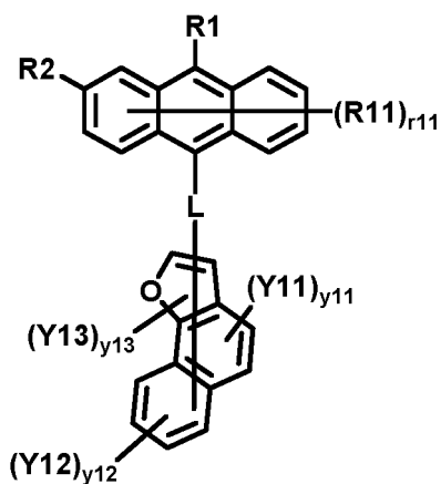
[Chemical Formula 1-6]
