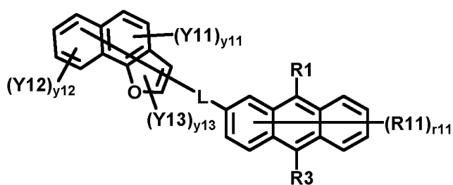
[Chemical Formula 1-6]
