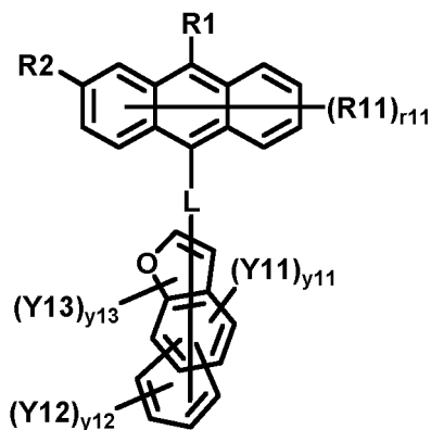
[Chemical Formula 1-3]
