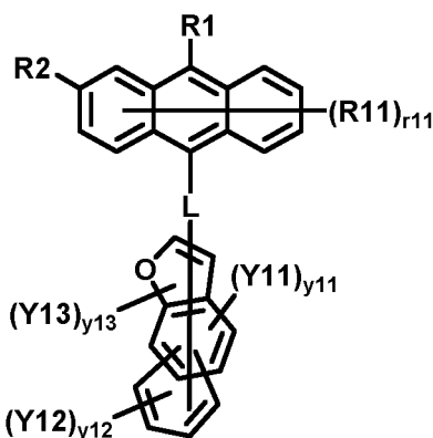
[Chemical Formula 1-3]
