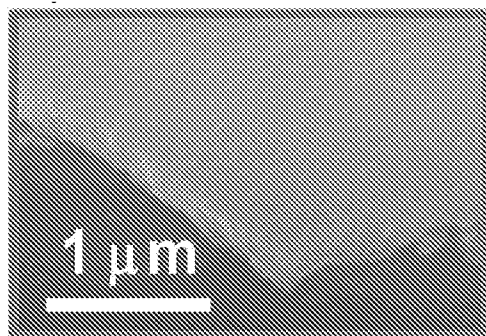
nanosheet
