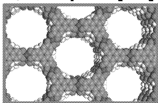
basal plane [004]
