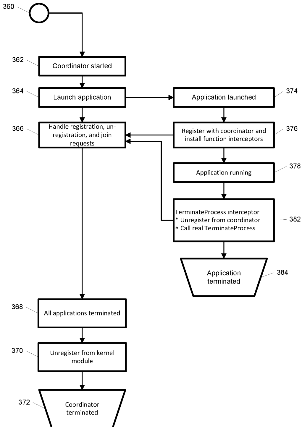
Fig 8. Removing an application from its application group
