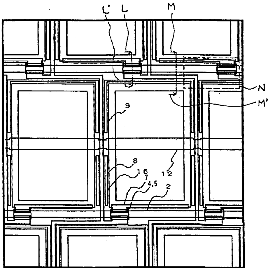
Fig. 11 PRIOR ART
