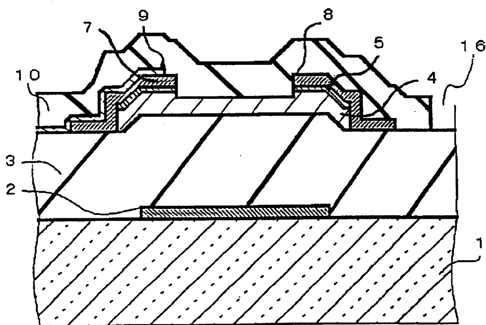
Fig. 12 PRIOR ART
