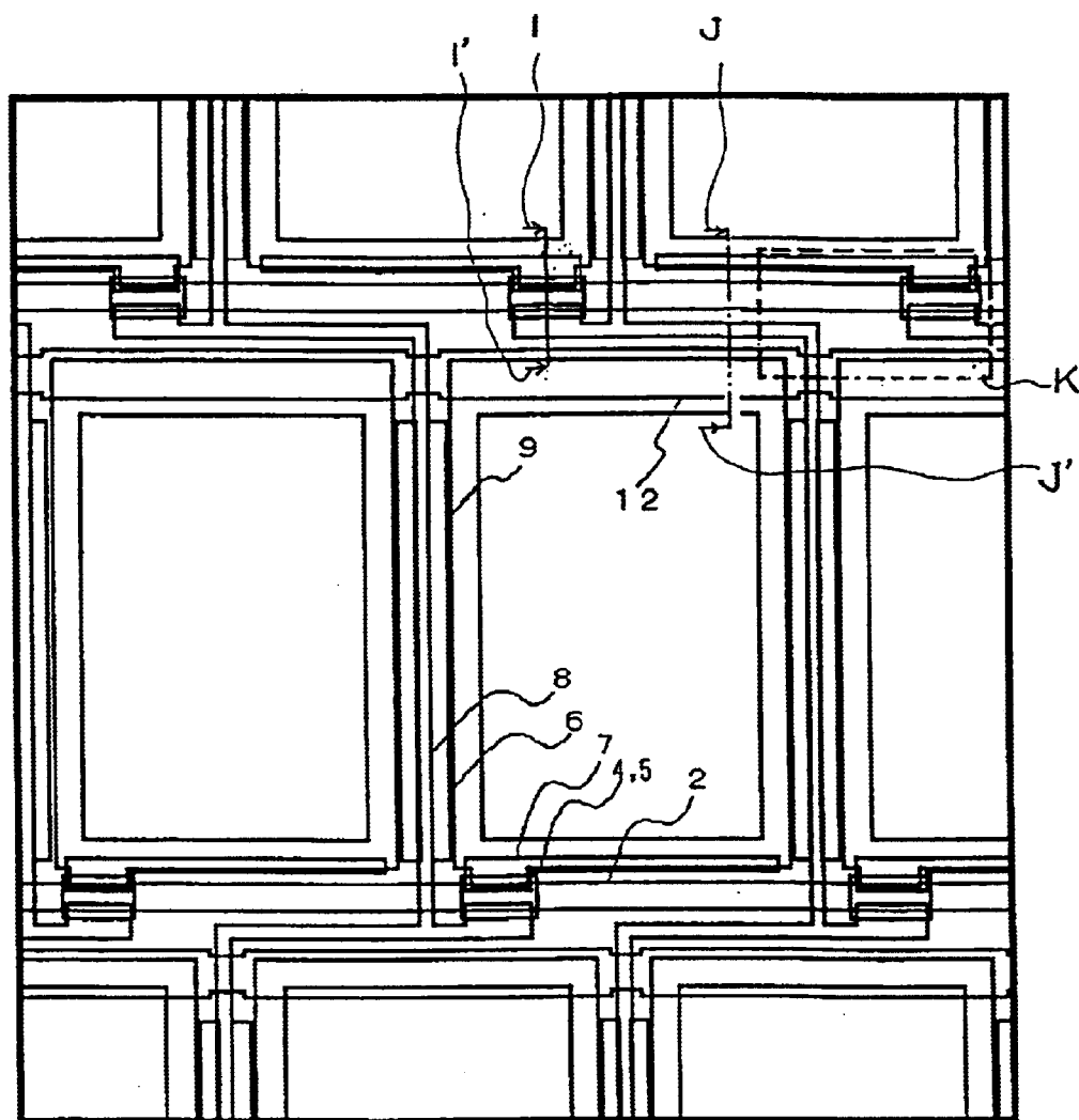
Fig. 6 PRIOR ART
