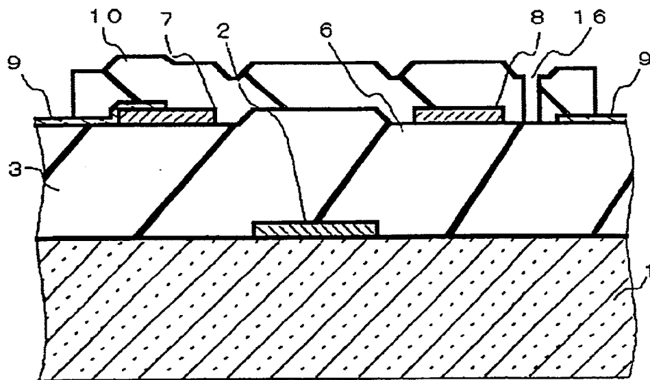
Fig. 13 PRIOR ART
