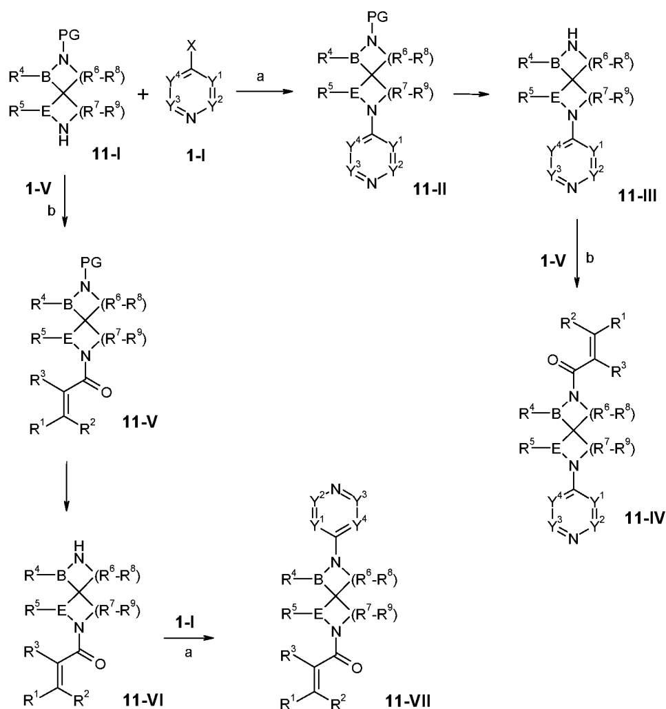
[449] Scheme 11:
