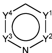
Formula (A)
