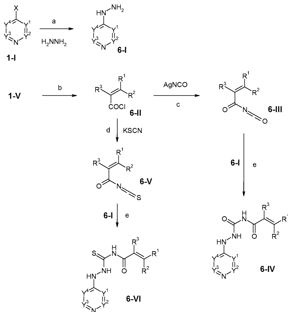
[432] Scheme 6:
