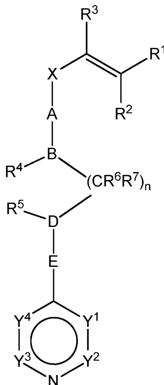
Formula (I)
