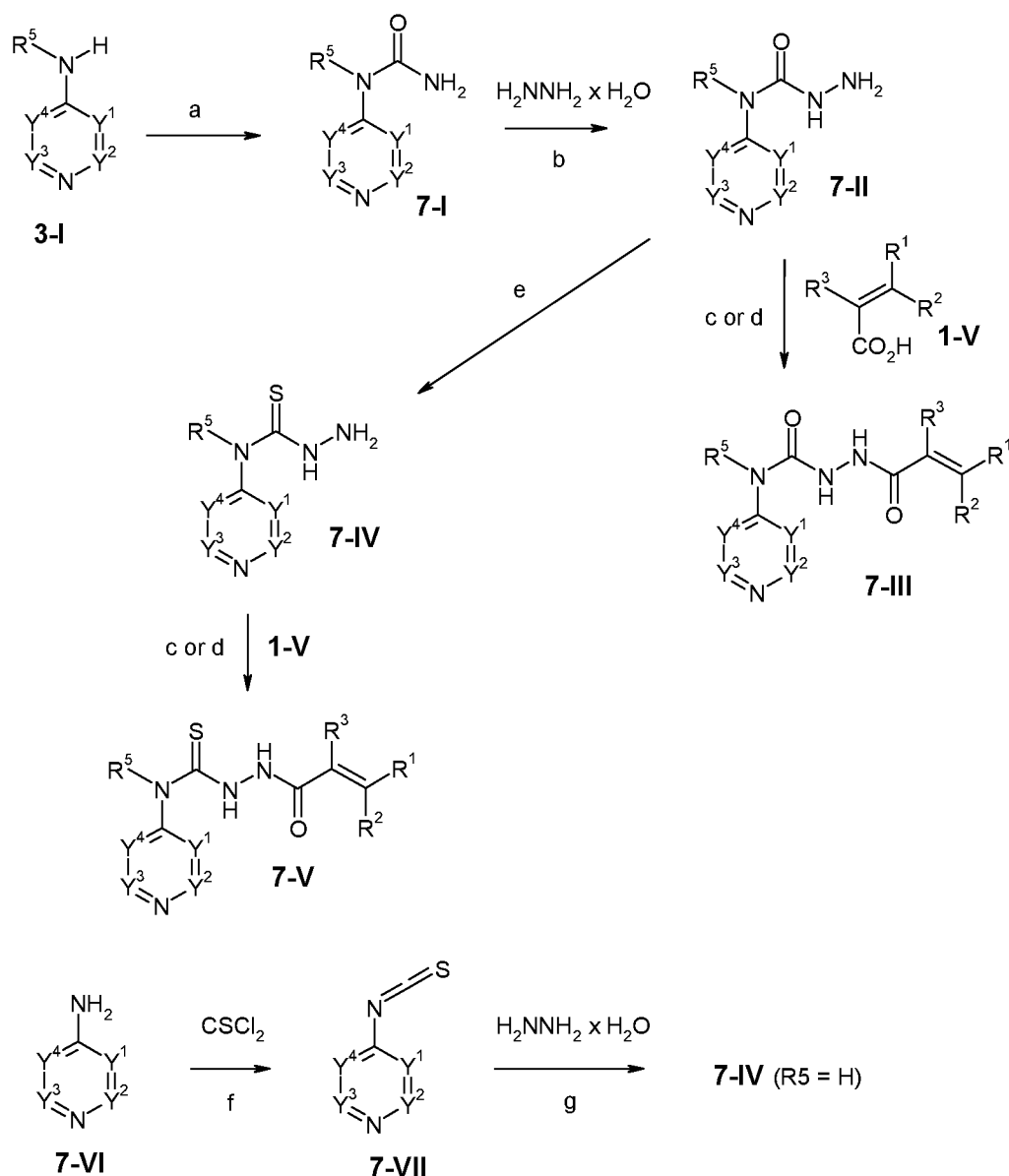
[435] Scheme 7:
