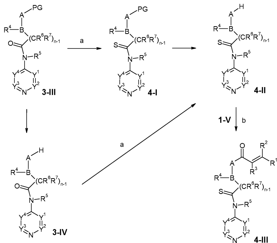
[425] Scheme 4:
