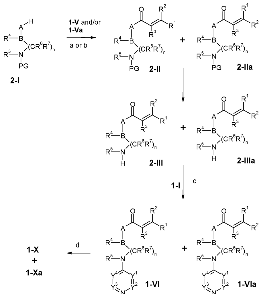
[418] Scheme 2:
