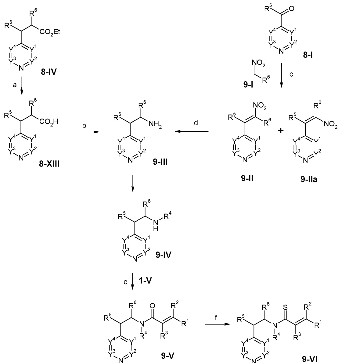
[442] Scheme 9:
