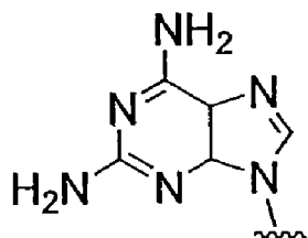
N9-(2,6,-diaminopurine)
