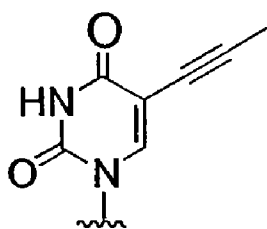
5-propynyl-U
