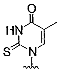
2-thio-T
