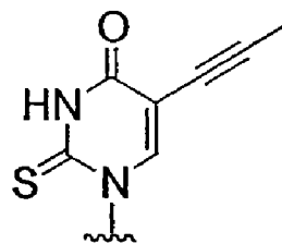
2-thio-5-propynyl-U
